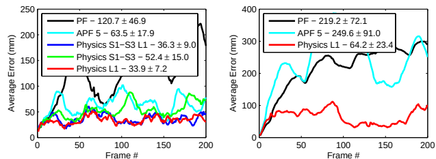
Figure 9. Quantitative Tracking Performance. Multi-view tracking performance of the proposed physics-based prior filtering method (Physics) with different training datasets versus standard Particle Filter (PF) and Annealed Particle Filter (APF 5) with 5 layers of annealing is shown on the left. Tracking performance using monocular sequence is analyzed on the right. In both cases L1 walking sequence was used; in the case of multi-view tracking with 4 cameras and 250 particles, in the case of monocular setup with single camera view and 1000 particles. See text for details.
