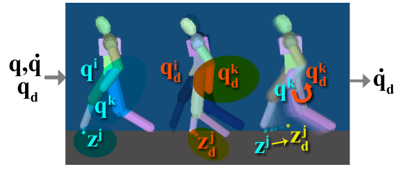
Figure 4. Motion Controller. Input kinematic pose \mathbf{q} determines the positions \mathbf{z}^j of markers on the feet (left), the desired kinematic pose \mathbf{q}_d their desired positions \mathbf{z}_d^j (middle). Desired positions are adjusted to prevent penetration with the ground and constraints on the marker velocities \dot{\mathbf{z}}^j and joint DOF derivatives \dot{\mathbf{q}}^k of the helper figure are formed (right). Superscripts i index the figure’s angular DOFs, superscripts j the markers and superscripts k the angular DOFs of the figure segments that have no markers j attached.
