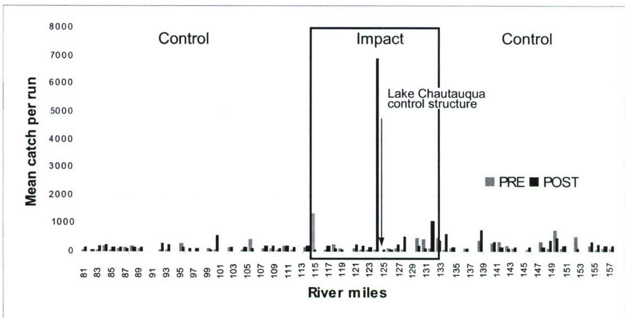
Figure 2. Day electrofishing mean catch per run for the pre- and post-Habitat Rehabilitation and Enhancement Project periods by Illinois River mile (pre-HREP mean catch = -55.564 + 1.878 \times \text{river mile} , n = 59 ; df = 1, 57 ; f = 2.328 ; P = 0.133 ; r^2 = 0.022 , post-HREP mean catch = -17.305 + 2.856 \times \text{river mile} , n = 59 ; df = 1, 57 ; f = 0.305 ; P = 0.583 ; r^2 = 0 ).
