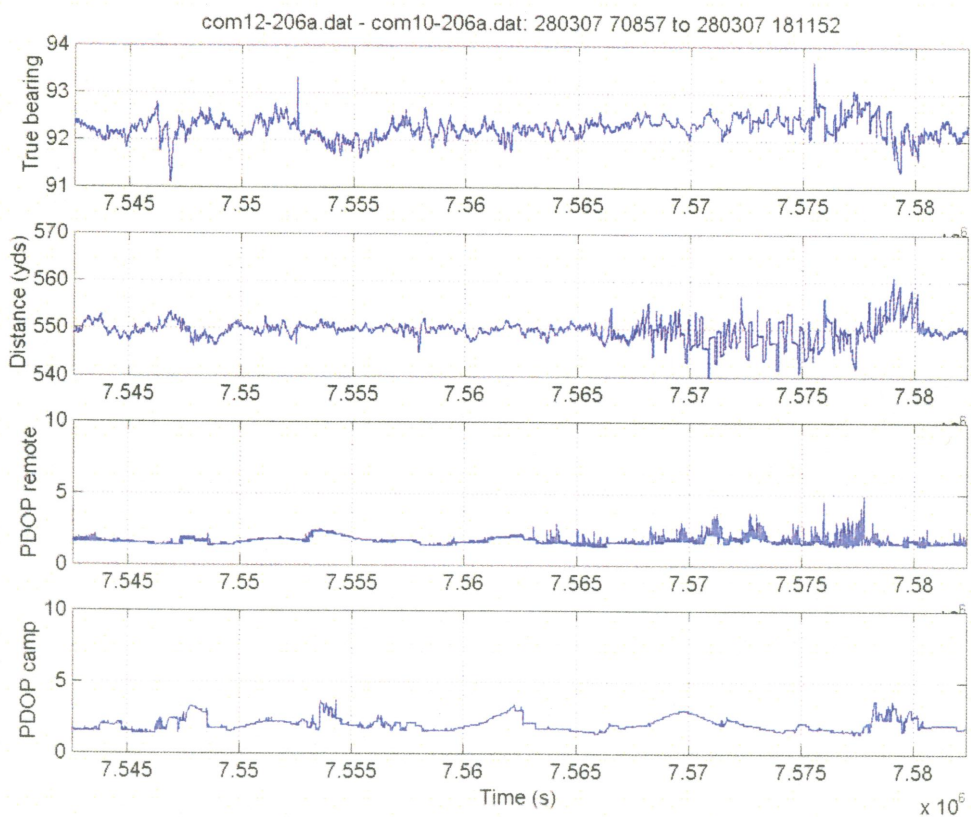
Figures C-1a, b. Range, bearing, & PDOP's between GPS's placed at hyd #1 & the (0,0). C-1a is from 3/26 and C-1b is 3/28.
