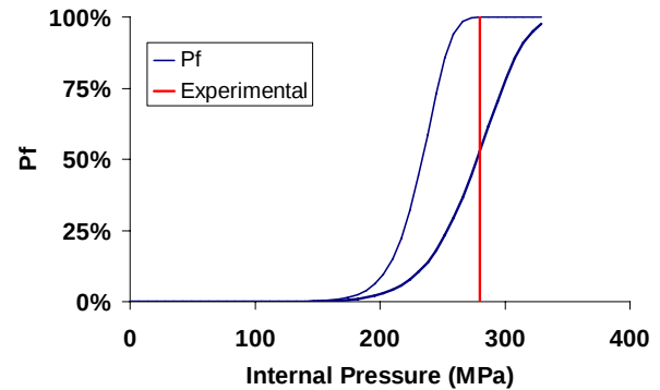
Figure 3 - High and low predictions for the burst pressure for a filament wound composite sheathed silicon nitride tube (SN47).
