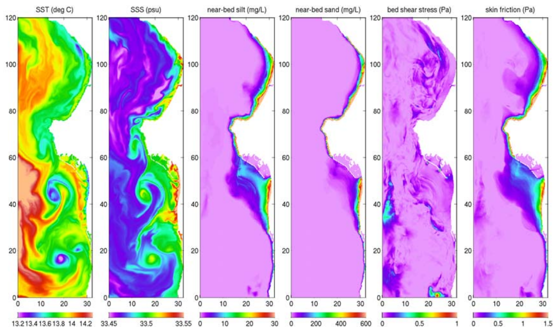
Figure 5. Instantaneous fields of sea-surface temperature, salinity, silt and sand, bed shear stress, and bed skin-friction shear stress from the high-resolution (200 m) Palos Verdes ROMS simulation embedded in the 1-km Southern California Bight grid.
