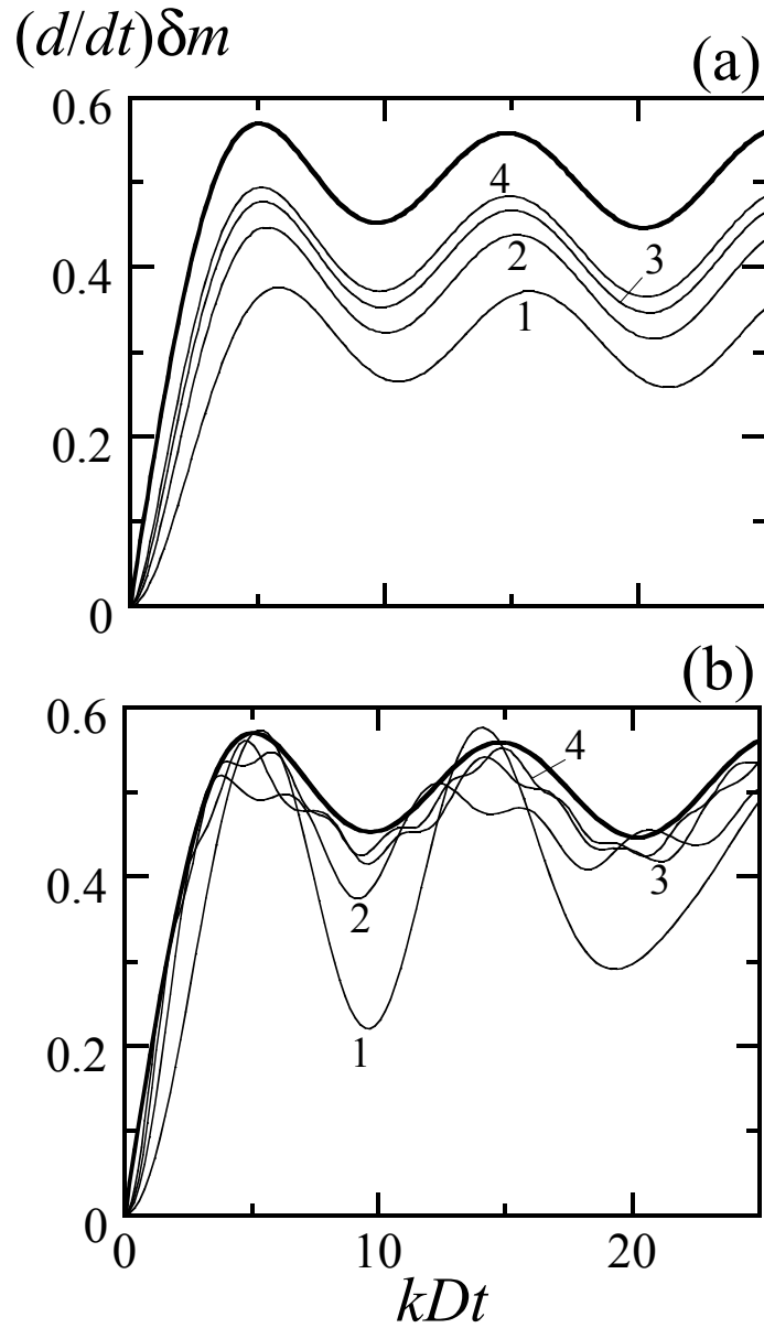
Figure 13. Normalized time derivatives of the areal mass modulation amplitude \delta m for surface ripples (thick lines), exponential (a) and Bessel-function (b) localized density perturbations in the target (thin lines, labeled by the value of the parameter q/k ) vs. normalized time kDt for g = 5/3 , M_1 = 10 .
