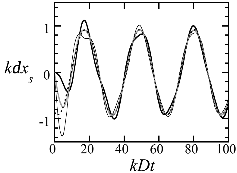
Figure 6. Normalized shock ripple amplitude kdx_s vs. normalized time kDt for the long-wavelength “quilt” case of the pre-shock density modulation, g = 5/3 , M_1 = 10 , k_x/k_y = 1/5 . Dotted line displays the asymptotic formula (35), thick, thin and gray solid lines correspond to the rigid piston, free surface and isolated shock boundary conditions, respectively.
