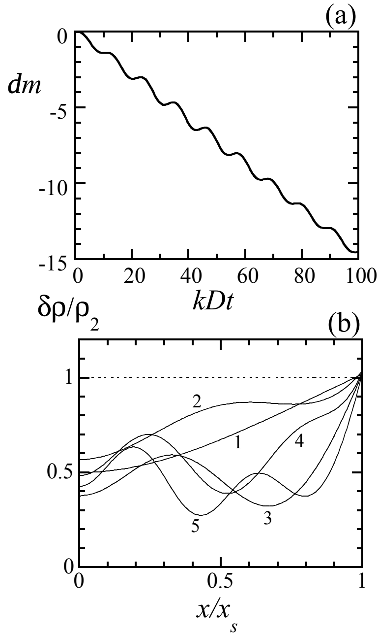
Figure 11. (a) Normalized areal mass modulation amplitude vs. normalized time kDt for the “stripes” pre-shock density perturbation, g = 5/3 , M_1 = 10 , rigid piston. (b) Relative post-shock density modulation amplitude profiles \tilde{r} = dr / r_2 shown at the times when the shock wave traveled 1, 2, 3, 4 and 5 lateral perturbation wavelengths (solid lines). Dotted horizontal line indicates the pre-shock relative density perturbation amplitude.
