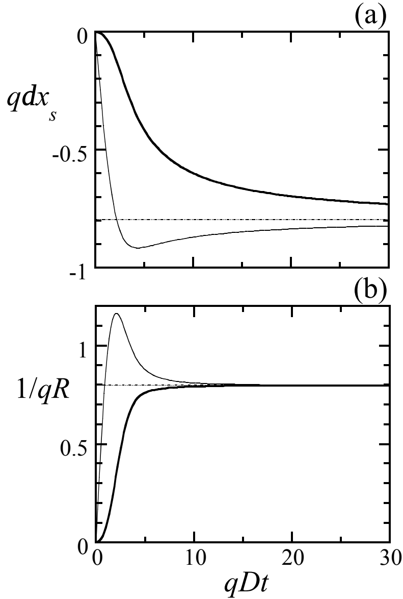
Figure 4. Normalized shock displacement amplitude qdx_s (a) and normalized curvature of the shock front 1/qR at r = 0 (b) vs. normalized time qDt for the cylindrical Gaussian “tube” localized pre-shock density perturbation, g = 5/3 , M_1 = 10 . Thick and thin solid lines correspond to the rigid piston and free surface boundary conditions at the piston surface, respectively. Horizontal dotted lines show the asymptotic values (60) and (61).
