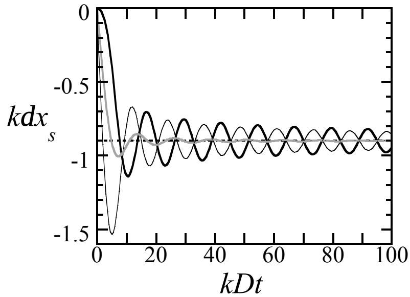
Figure 3. Normalized shock ripple amplitude kdx_s vs. normalized time kDt for the “stripes” case of the pre-shock density modulation, g = 5/3 , M_1 = 10 . Dotted line displays the asymptotic value (34), thick, thin and gray solid lines correspond to the rigid piston, free surface and isolated shock boundary conditions, respectively.
