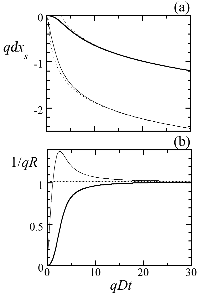
Figure 5. Normalized shock displacement amplitude qdx_s (a) and normalized curvature of the shock front 1/qR at y = 0 (b) vs. normalized time qDt for the planar Gaussian “joint” localized pre-shock density perturbation, g = 5/3 , M_1 = 10 . Thick and thin solid lines correspond to the rigid piston and free surface boundary conditions at the piston surface, respectively. Dotted lines in (a) show the asymptotic formulae (66) for each boundary condition; horizontal dotted line in (b) shows the asymptotic curvature (67).
