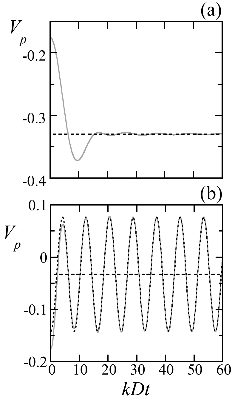
Figure 9. Longitudinal velocity perturbation amplitude at x = 0 vs. normalized time kDt for an isolated shock wave interacting with a “quilt” pre-shock density perturbation shown as gray line. (a) Long-wavelength regime, k_x/k_y = 1/5 ; horizontal dashed line – late-time asymptotic value given by (88). (b) Short-wavelength regime, k_x/k_y = 1 ; dotted line - late-time asymptotic oscillations given by (91), horizontal dashed line – average late-time value given by (88). For both cases, g = 5/3 , M_1 = 10 .
