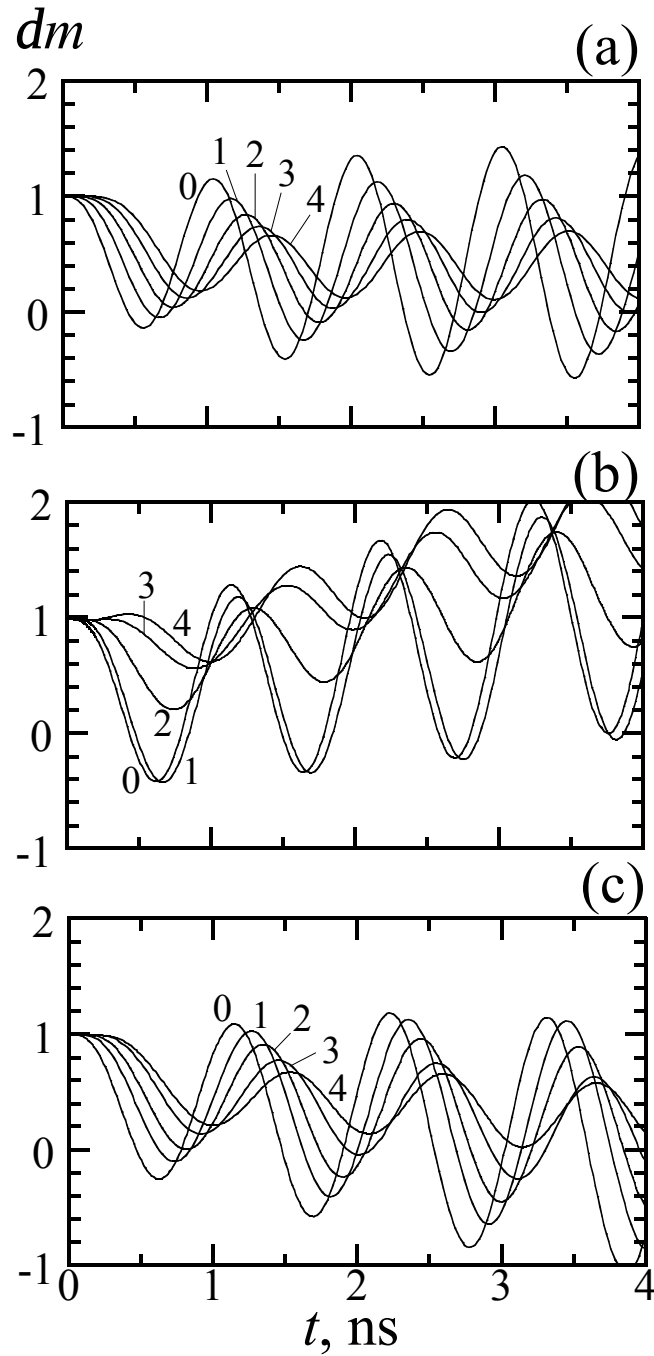
Figure 15. Normalized areal mass modulation amplitude dm vs. time for density modulation profiles (97) localized near the surface: g = 5/3 , M_1 = 10 , lateral perturbation wavelength l = 2p/q = 30 \text{ } \mu\text{m} , rigid piston velocity V_p = 4 \times 10^6 \text{ cm/s} ; in the simulations, effective ripple amplitude dx_0 = 0.1 \text{ } \mu\text{m} : (a) theory, (b) simulation with constant time step, (c) simulations with initially reduced time step. Lines 0 through 4 are indexed by the value of the parameter n in (97).
