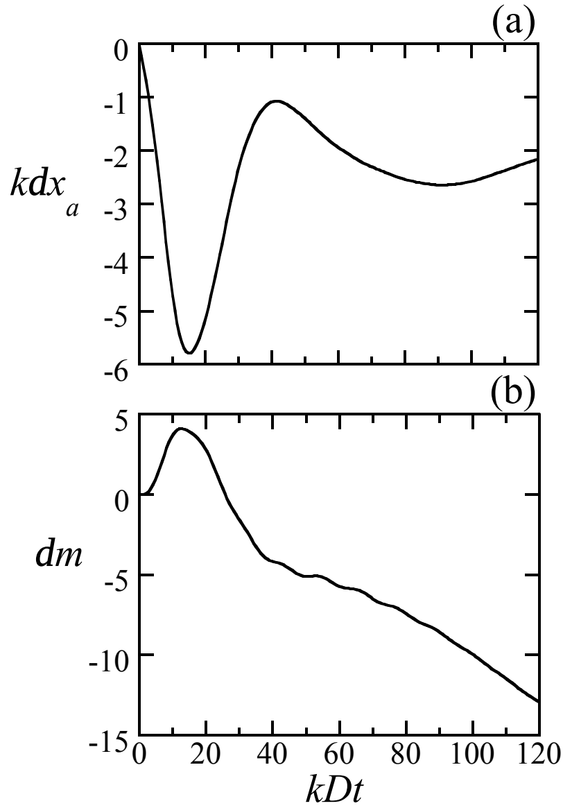
Figure 12. Normalized displacement of the ablation front kdx_a (a) and areal mass modulation amplitude dm (b) vs. normalized time kDt for a “stripes” density perturbation g = 5/3 , M_1 = 10 , and an ablation front with r_D = 0.0625 , M_a = 0.05 acting as a piston.
