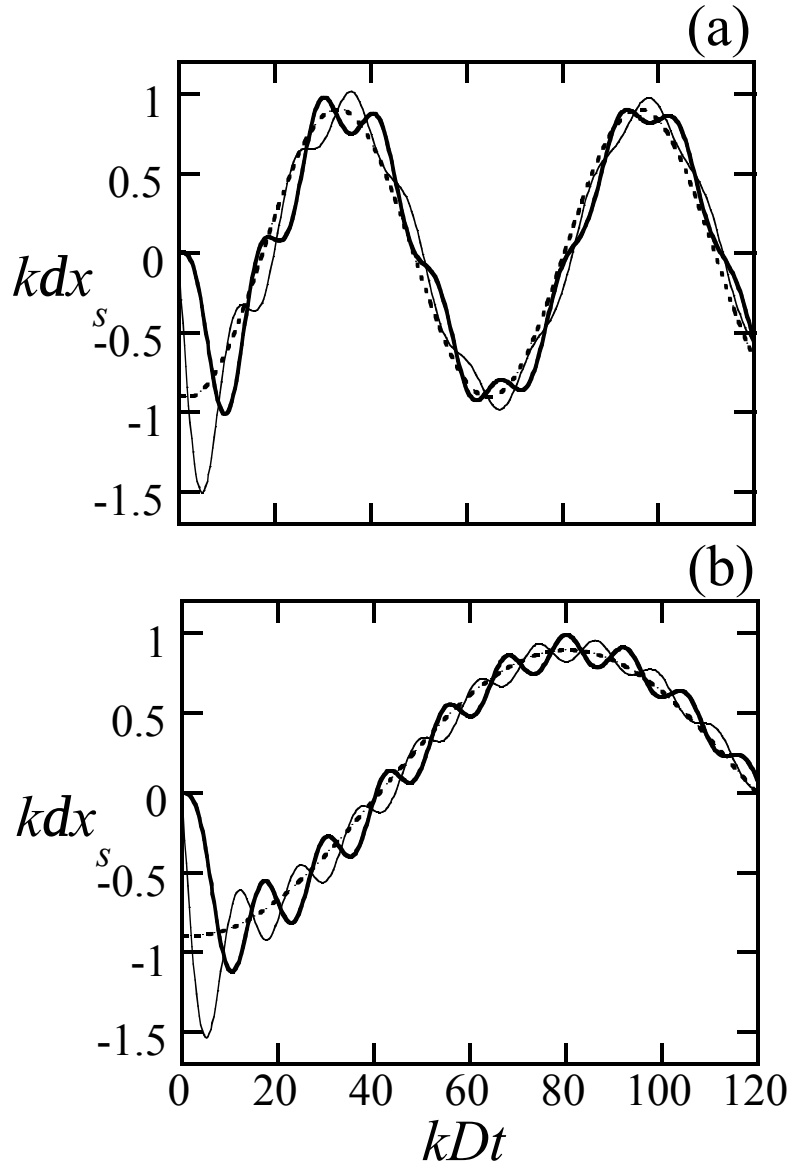
Figure 8. Normalized shock ripple amplitude kdx_s vs. normalized time kDt for the pre-shock standing sonic wave, g = 5/3 , M_1 = 10 (a) and M_1 = 25 (b). Dotted line displays the asymptotic shape (32), thick and thin solid lines correspond to the rigid piston and free surface boundary conditions at the piston surface, respectively.
