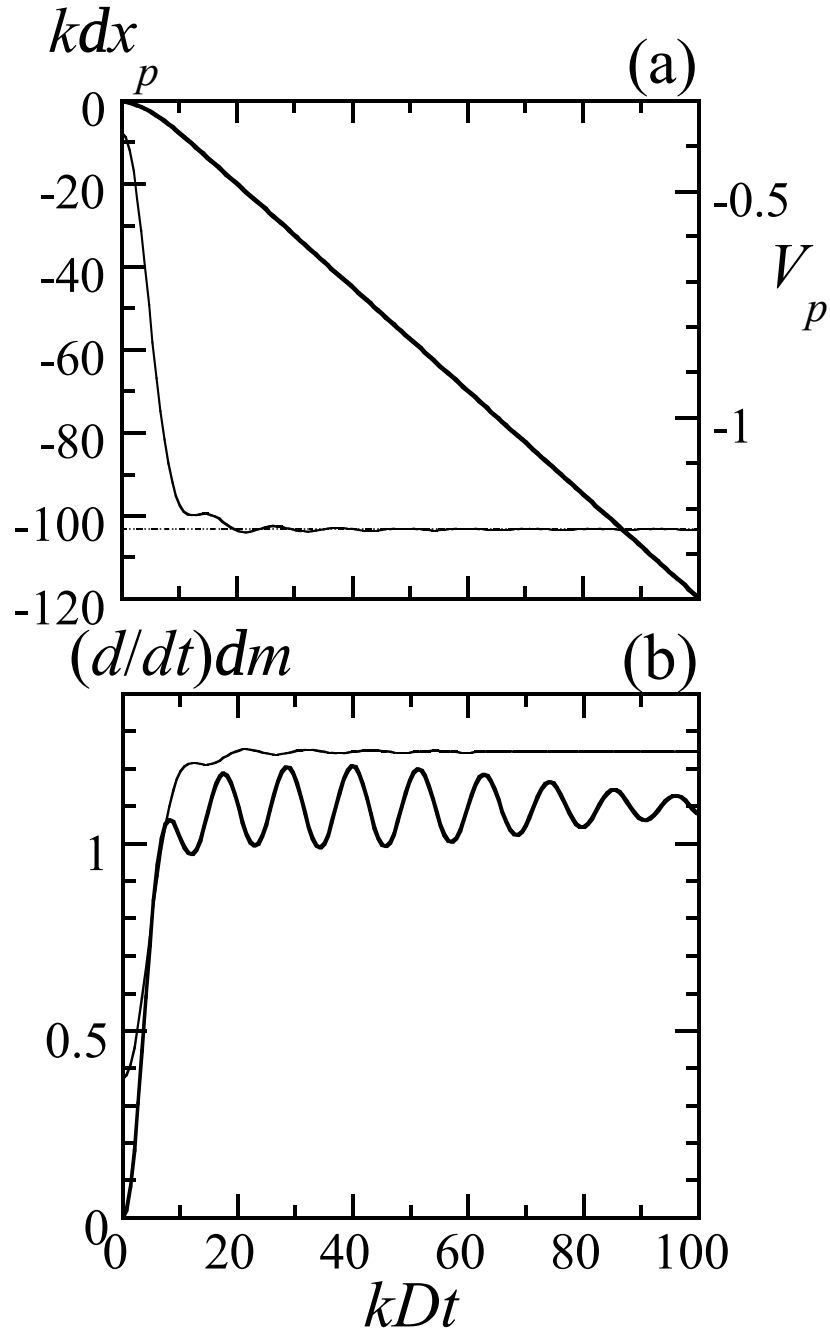
Figure 10. Normalized displacement amplitude of the piston surface kdx_p (thick), its time derivative V_p (thin), and the constant asymptotic value (88) (horizontal dashed line) (a); time derivative of areal mass modulation amplitude dm (thick) and contribution to it due to the surface ripple (thin line) (b) vs. normalized time kDt for the “stripes” pre-shock density perturbation, g = 5/3 , M_1 = 10 , free surface boundary conditions at the piston.
