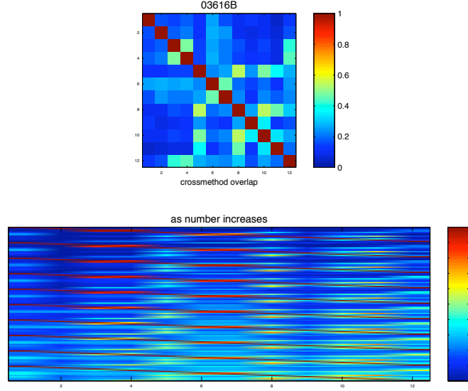
Figure 2.42: Same as Figure 2.38, for dataset D5.
