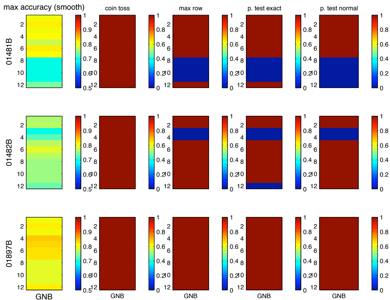
Figure 2.1: Comparison of result significance under various null models, for subjects in dataset D1 (rows). The first column contains the accuracy results using the best number of voxels selected with each of the 12 methods. The remaining columns contain the significance of the results in the first column under each of the null models (red is significant, blue is not).
