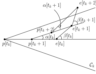
Fig. 16. Illustrating Lemma IV.6. This is a case of the evader moving out of the cone sector sequence C_k by moving out of C_{k,0} .
