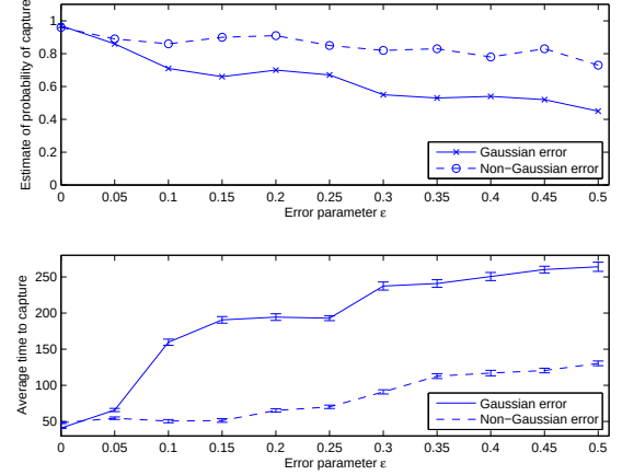
Fig. 22. Effect of measurement noise in the single pursuer problem. For a particular evader strategy, we study how the capture probability and average capture time given that the strategy succeeds, vary with the noise parameter \epsilon , under Gaussian and Non-gaussian error models. In the top figure, an interval of \pm 0.1 (not shown to preserve clarity) about the probability estimates is the 95% confidence interval given by [P(\epsilon) - 2\sqrt{\frac{0.25}{n}}, P(\epsilon) + 2\sqrt{\frac{0.25}{n}}] , where n = 100 is the number of trials [23]. In the bottom figure, the vertical bars give a 95% confidence interval about the average capture time T(\epsilon) which is given by [T(\epsilon) - 2\sqrt{\frac{SD(\epsilon)}{nP(\epsilon)}}, T(\epsilon) + 2\sqrt{\frac{SD(\epsilon)}{nP(\epsilon)}}] , where SD(\epsilon) is the standard deviation in the capture time, P(\epsilon) is the estimated probability of success and n = 100 is the number of trials [23].
