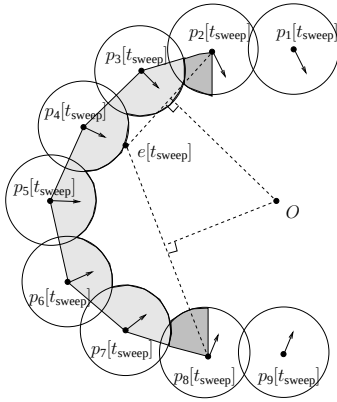
Fig. 7. Multiple pursuer problem: CIRCUMCENTER strategy. At time t_{\text{sweep}} , the evader position is sensed by p_4 . Pursuers p_2, \dots, p_8 move towards O , the circumcenter of triangle formed by p_2 , e and p_8 . p_1 and p_9 move parallel to p_2 and p_8 respectively. The circles around the pursuers represent their sensing discs.
