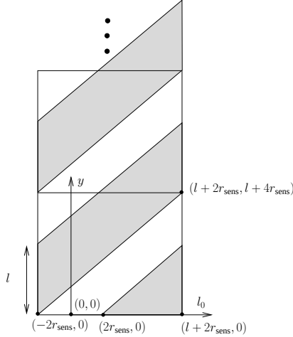
Fig. 19. The region of integration in determining P(e \in S) in the proof of Theorem III.7. Fix a value of l_0 in the interval (-2r_{\text{sens}}, l + 2r_{\text{sens}}) to get the values of y that correspond to P(e \in S) .
