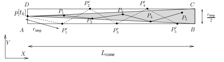
Fig. 14. Upper bound on the number of steps a pursuer can be inside a cone sector. The cone sector C_{k,0} is illustrated here. The dotted path shows a hypothetical pursuer path that takes the maximum number of steps before leaving a cone sector.
