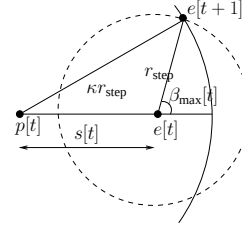
Fig. 15. Constraint on maximum evasion angle. The dotted circle represent the evader's motion disc. The circle centered at p[t] (shown partially here) is the pursuer's sensing range.
