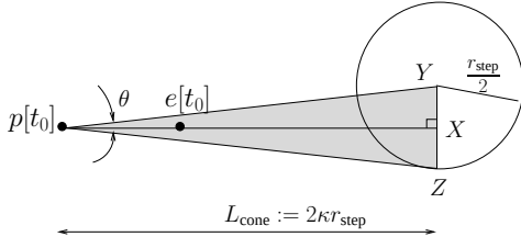
Fig. 12. Construction of cone C_{0,0} . Choose X on the line e[t_0]p[t_0] such that \|p[t_0] - X\| = 2\kappa r_{\text{step}} . YZ has length \frac{r_{\text{step}}}{2} and is perpendicular to segment p[t_0]X with X as its midpoint. \theta is the cone angle.
