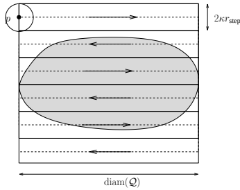
Fig. 10. A hypothetical sweeping path to determine upper bound on number of steps to detect the evader.
