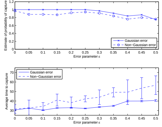
Fig. 25. Effect of measurement noise in the multiple pursuer problem. For a particular evader strategy, we study how the capture probability (top figure) and average capture time (bottom figure) given that the strategy succeeds, vary with the noise parameter \epsilon , under Gaussian and Non-gaussian error models. The error bars are in accordance with Figure 22.
