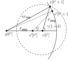
Fig. 17. Illustrating parameters in Equation (18). e'[t^*] is a point such that \|p[t^*] - e'[t^*]\| = r_{\text{step}} . \gamma is the value of the maximum evasion angle if the evader were at e'[t^*] . The circle of radius \kappa r_{\text{step}} around the pursuer (shown partially here) is the pursuer's sensing disc which the dotted circle around e[t^*] is the evader's motion disc.
