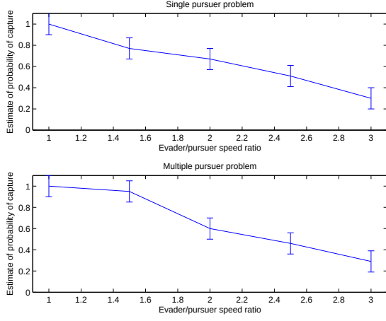
Fig. 24. Performance of Sweep-Pursuit-Capture strategy against a faster evader. For a particular evader strategy, we study how the capture probability varies for higher evader speeds, assuming no measurement noise. The top figure presents the single pursuer case and the bottom figure presents the multiple pursuer case. The error bars are in accordance with Figure 22.
