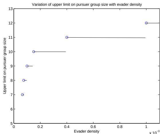
Fig. 27. Plot of maximum group size of pursuers that can be sustained versus the evader density \delta , for \kappa = 5 , r_{\text{step}} = 1 , \nu = 10000 .
