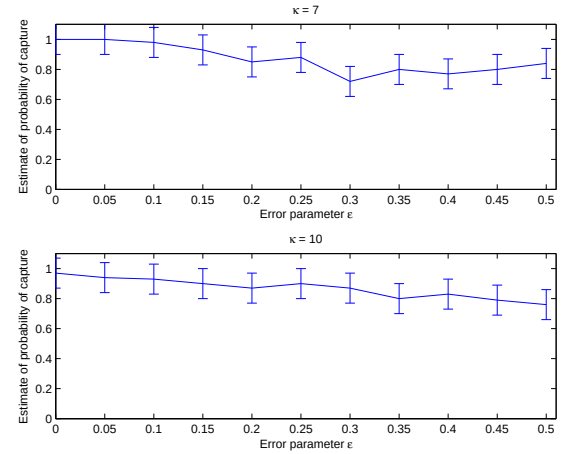
Fig. 23. Effect of varying the sensing to stepping radius ratio \kappa in the single pursuer problem. For a particular evader strategy, we study how the capture probability varies for \kappa = 7 and \kappa = 10 with the noise parameter \epsilon , under Gaussian noise model. The error bars are in accordance with Figure 22.
