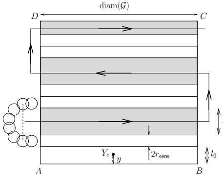
Fig. 18. Illustrating the proof of Theorem III.7.
