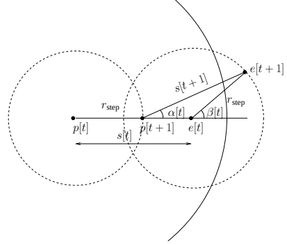
Fig. 11. Relation between the deviation angle \alpha[t] and the evasion angle \beta[t] . The dotted circles represent the motion discs of the players. The circle centered at p[t] (shown partially here) is the pursuer's sensing range.
