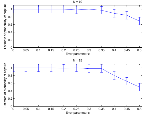
Fig. 26. Effect of varying the number of pursuers N in the multiple pursuer problem. For a particular evader strategy, we study how the capture probability varies for N = 10 and N = 15 with the noise parameter \epsilon , under Gaussian noise model. The error bars are in accordance with Figure 22.
