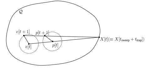
Fig. 4. Single pursuer problem: Using the LION strategy to capture the evader. The dotted circles represent the motion discs of the players.
