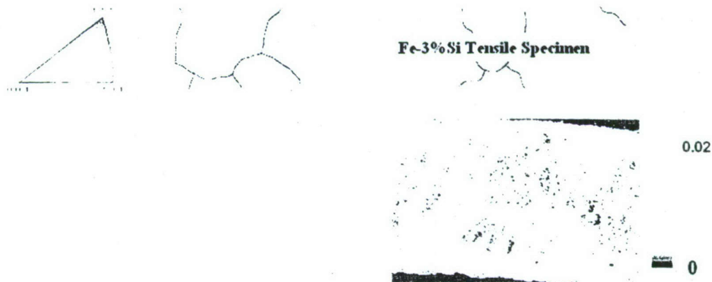
Figure 6 – First example of simulated (left) and measured (right) lattice curvature for a coarse-grained, columnar tensile Fe-3%Si specimen after straining to 20% strain. The simulated and measured maximum lattice curvatures agree within 20%.
