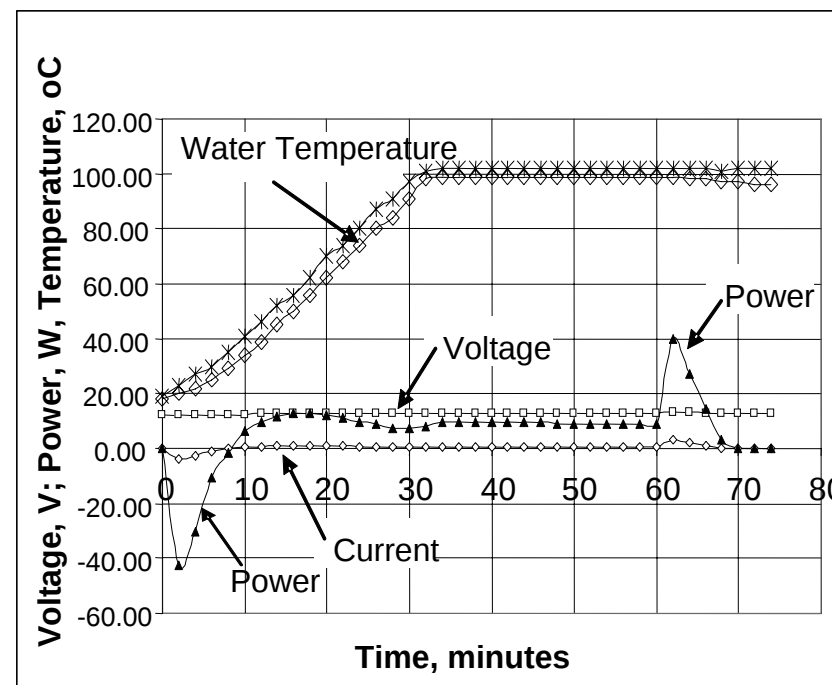
Self-Powered TRH Performance Test
