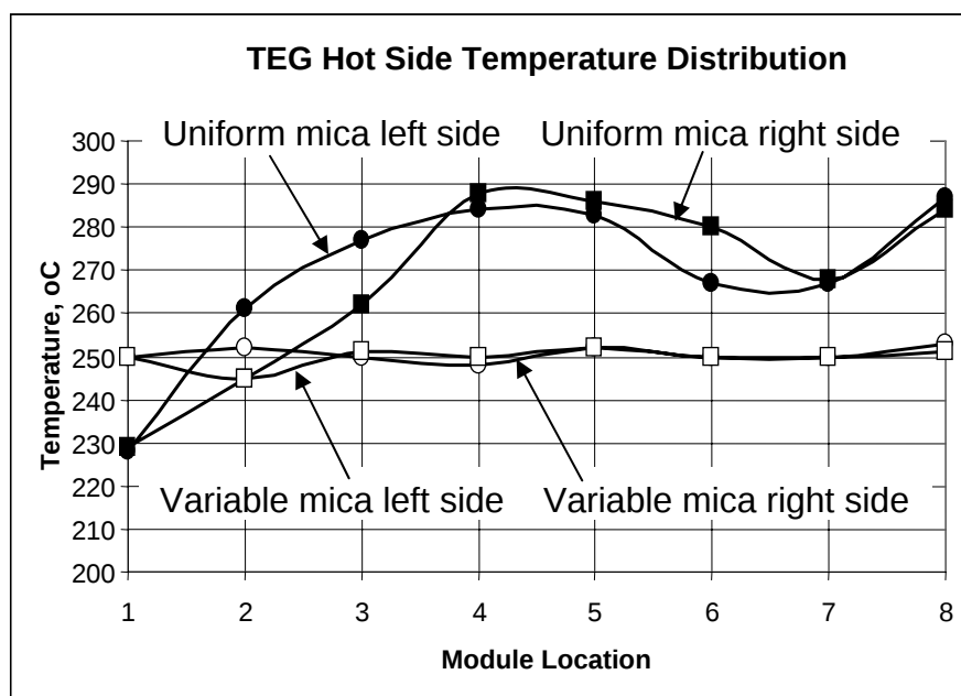
Hot side temperature distribution before and after temperature adjustment
