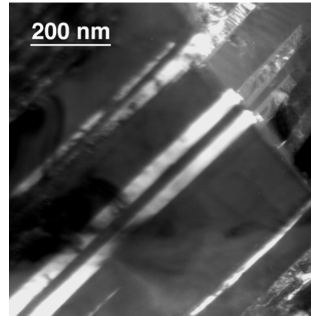
Deformation Twinning
