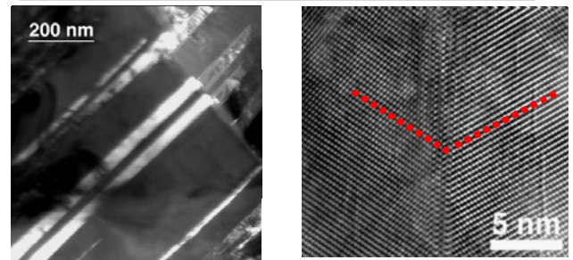
(a) (b) Figure 13. TEMs of 7.8 GPa sample
