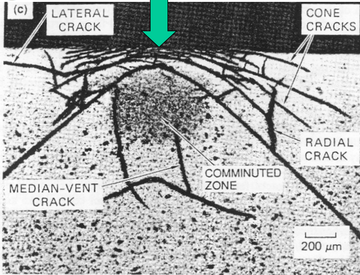
FIG. 8. Sectional views of subsurface cracking pattern in HP \text{Si}_3\text{N}_4 impacted by 2.4 mm diameter steel spheres at velocities of 56.4 \text{ m s}^{-1} (a) and 231 \text{ m s}^{-1} (b) and by a 2.4 mm diameter tungsten carbide sphere at 231 \text{ m s}^{-1} (c).
