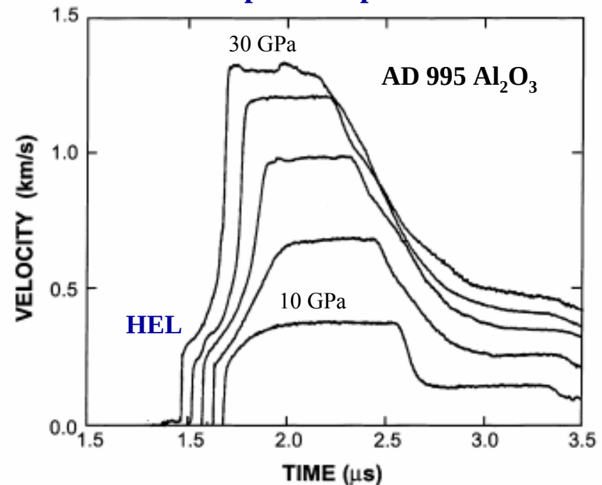
Shock compression profiles
