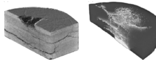
Reconstructed (left) virtual three-dimensional solid view and virtual (right) damage distribution within the target.
