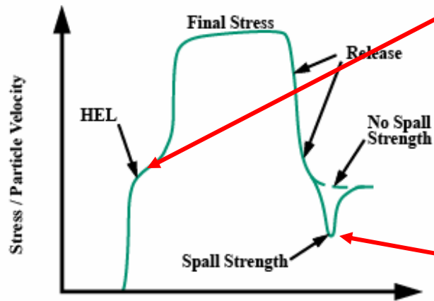
Schematic Plate Impact Hugoniot Curve
