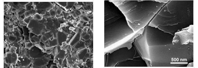
(a) (b) Figure 12. SEMs of 7.8 GPa sample
