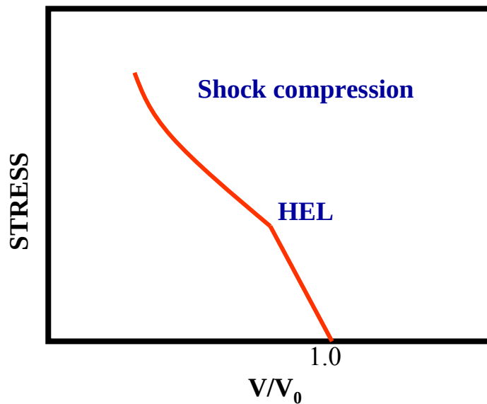
Stress-volume trajectory
