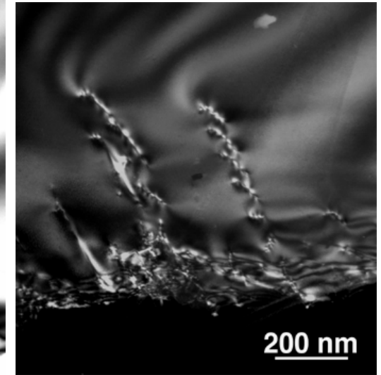
Dark-Field Image
