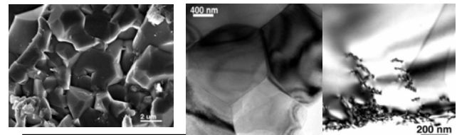
(a) (b) (c) Figure 11. SEM and TEMs of 6 GPa sample: a.) SEM in uncracked area; b.) TEM in uncracked area and c.) TEM in cracked area
