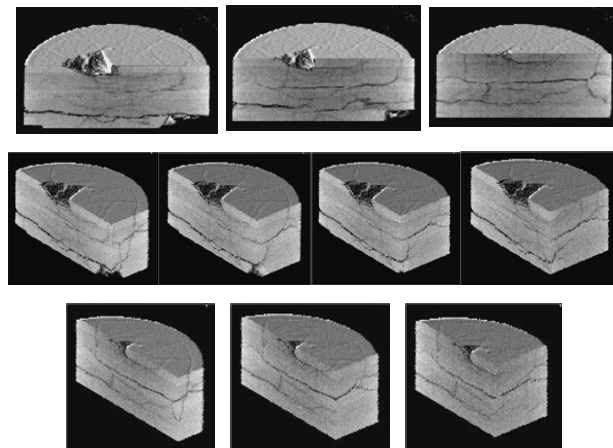
Figure 9. Three-Dimensional (3-D) virtual solid images of 6 GPa sample with sections cut away
