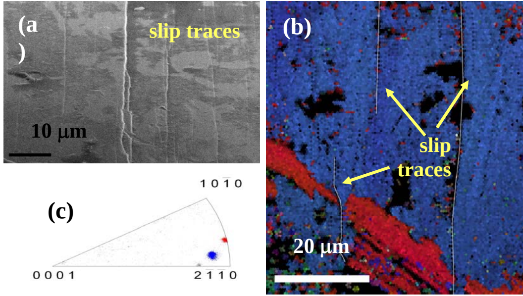
Figure 23. (a) SEM image showing intense slip bands on the surface of the \beta - processed sample (b) OIM map of a similar area showing the adjacent colonies in colors and the slip band propagation within and © inverse pole figure display the colony orientations
