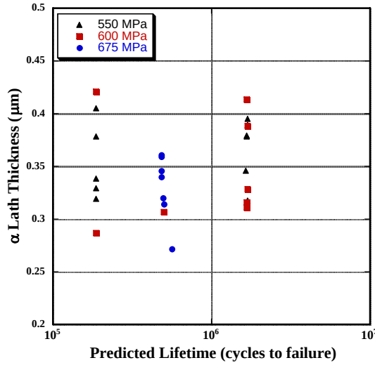
Figure 8. \alpha lath thickness versus predicted lifetime; data separated by stress.
