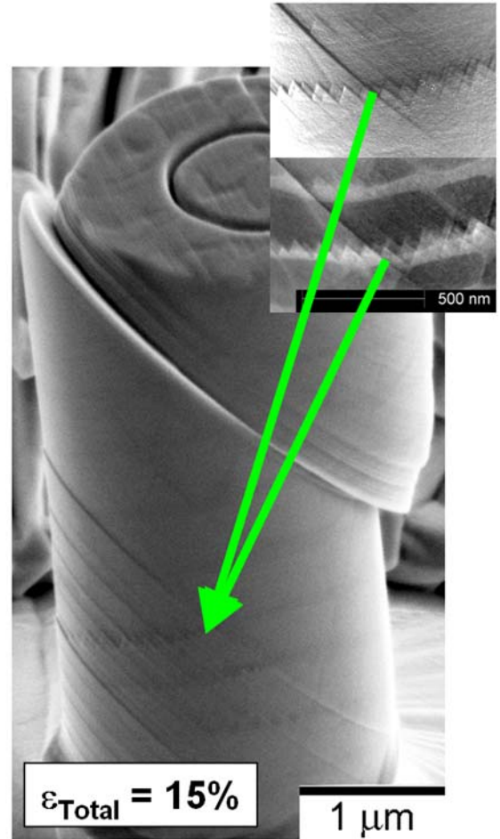
Figure 12. Images of ‘zig-zag’ slip in \langle 1\ 2\ 3 \rangle oriented 2.5 \mu\text{m} diameter compression samples. The upper inset image is a secondary electron image while the lower inset is a backscatter electron image.
