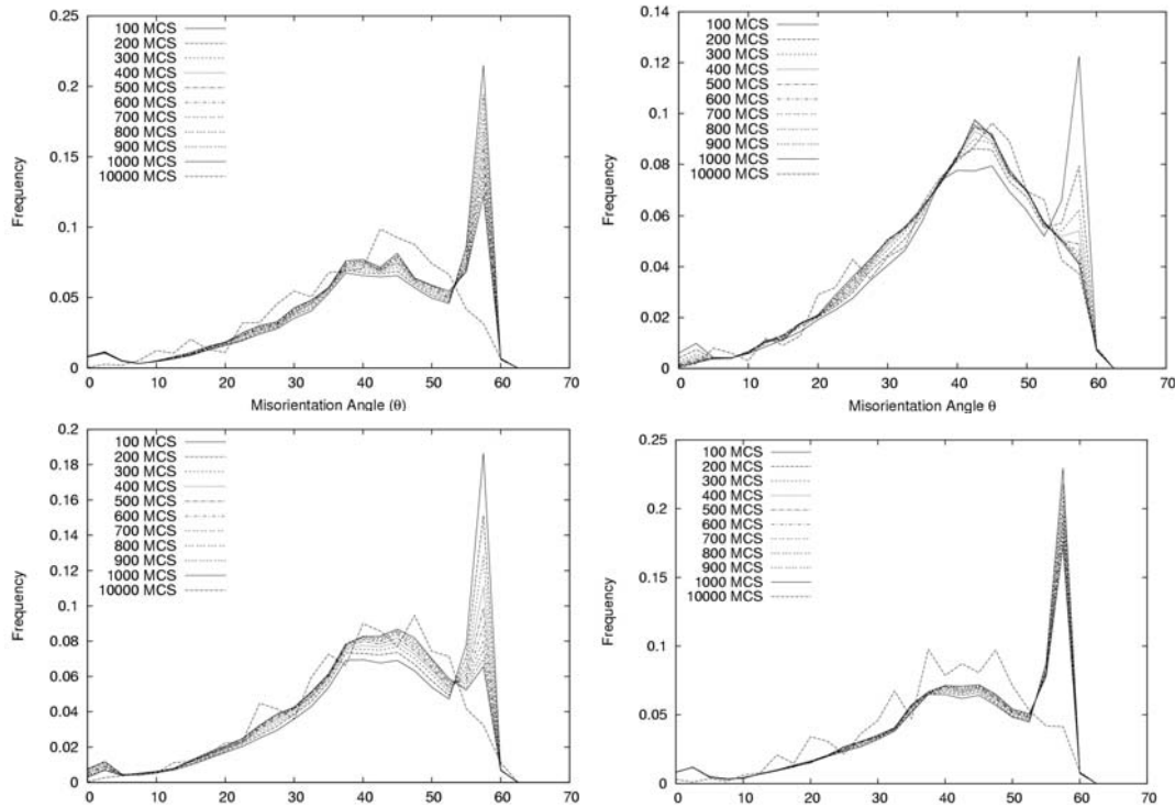
Figure 24. Misorientation distribution (MDF) as a function of time for a 0.04V_V and 30% of particles on grain boundaries a) R_0 = 7.6 b) R_0 = 11.2 c) R_0 = 15.2 d) R_0 = 18.4
