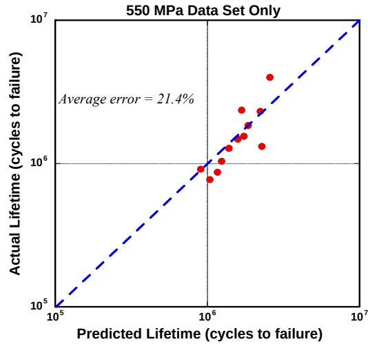
Figure 11b. Actual lifetime vs. Predicted lifetime for samples tested at 550 MPa.
