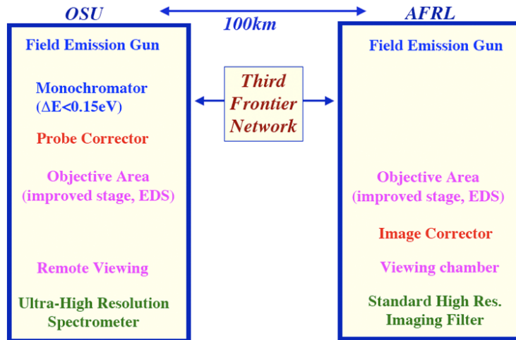
Figure 1. OSU/AFRL Microscope Concept
