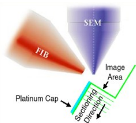
Figure 2: Schematic of serial sectioning with a DB-FIB-SEM.
