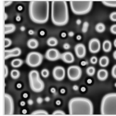
Figure 7. Typical tri-modal \gamma/\gamma' microstructures obtained in (a) experiment and (b) Ni-Al by phase field simulations that account for both heterogeneous and homogeneous nucleation mechanisms under continuous cooling conditions.
