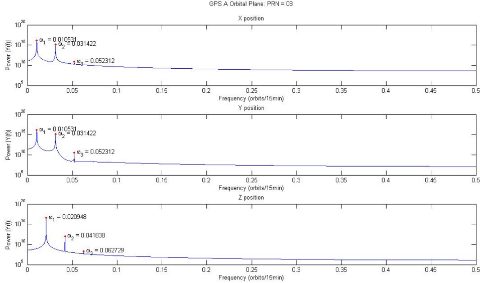
Figure 4.1: Frequencies of positions for PRN 08 located in the A orbital plane
