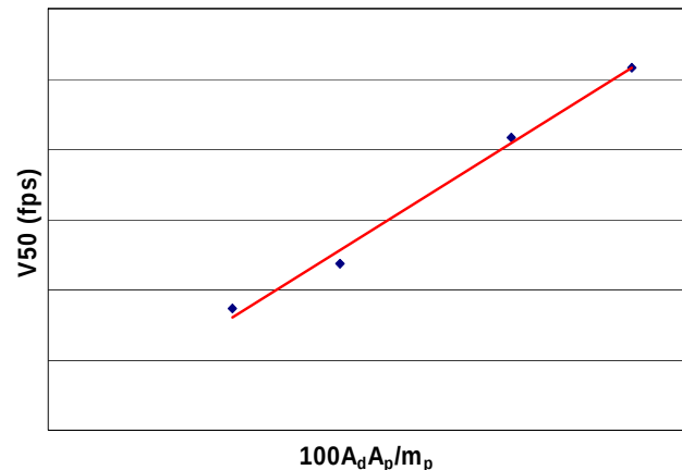
Fig. 6. V50 versus dimensionless parameter (trendline also shown)
