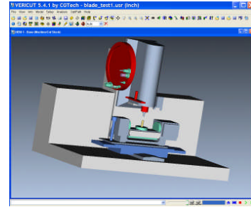
Figure 13, G-code Simulation.
