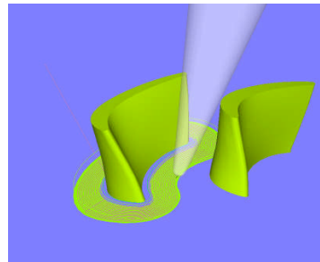
Figure 11, Mastercam Programming.
