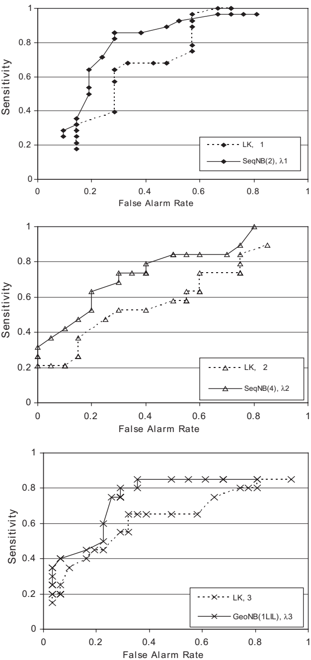
Fig. 1. ROC curve for the \lambda family.
