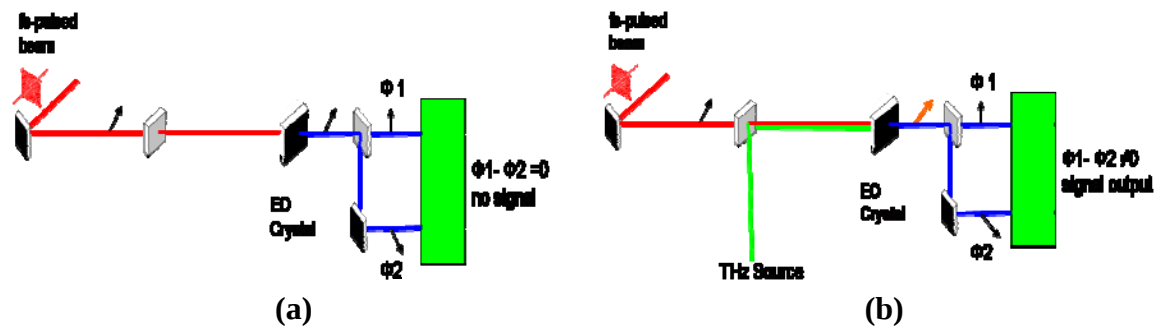
Figure 7. (a) Nirvana with no signal output and (b) Nirvana signal output due to THz
