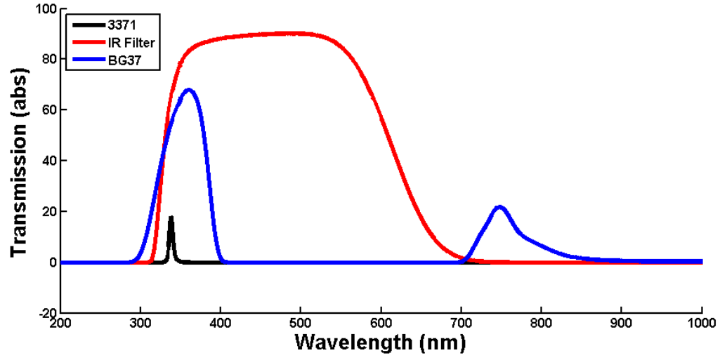
Figure 11. PMT filter performance comparison
