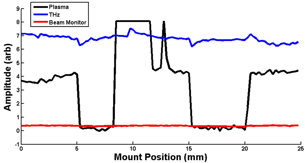
Figure 29. No change in THz detector signal with plasma on-off
