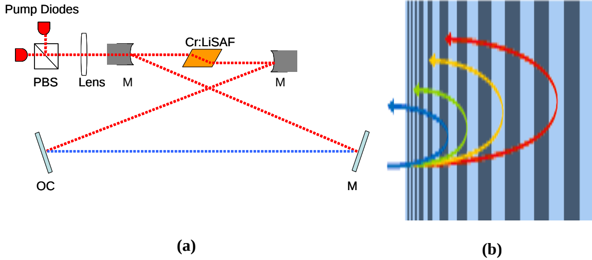
Figure 4. (a) Diode-pumped Cr:LiSAF cavity and (b) “double-chirped” mirror
