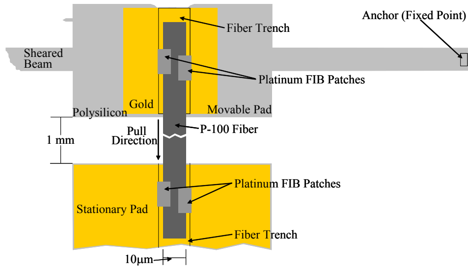
Figure 4-27: Illustration of reaction force mechanism for one test location of a 1000\ \mu\text{m} long carbon fiber.
