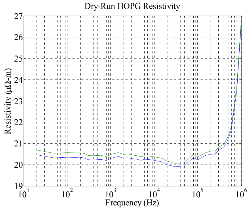
Figure 6-15: HOPG dry-run resistivity results for 500\ \mu\text{m} \times 1750\ \mu\text{m} strip of HOPG over two successive frequency sweeps.
