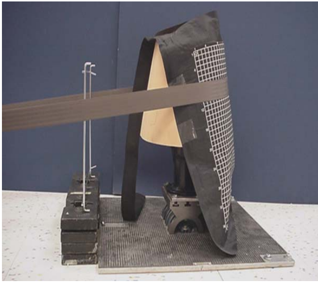
Figure 4. Set up for Hip Model Testing using the XSENSOR ® pad.
