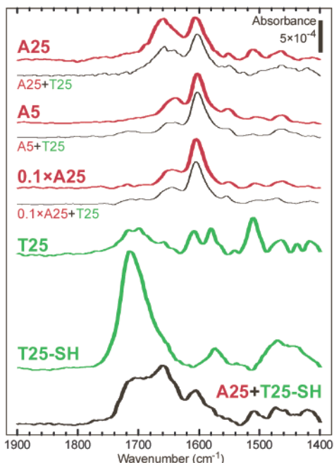
Figure 2. FTIR spectra of ssDNA films on Au following competitive adsorption from mixtures of (dA) n and (dT) n . Spectra for (dA) 25 + (dT) 25 , (dA) 5 + (dT) 25 , 0.1 × (dA) 25 + (dT) 25 , and (dA) 25 + (dT) 25 -SH mixtures are shown. The spectra following adsorption of (dA) 25 , (dA) 5 , 0.1 × (dA) 25 , (dT) 25 , and (dT) 25 -SH alone are shown for reference.
