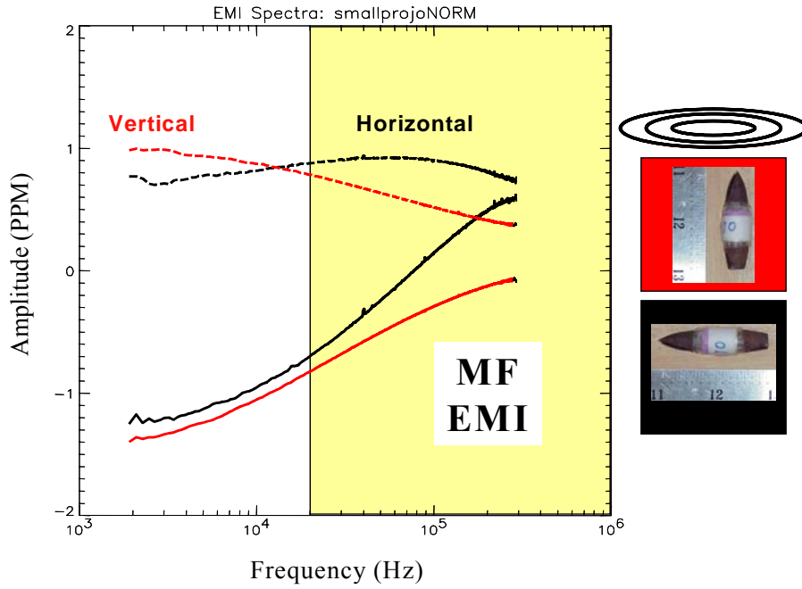
Figure 90. Measured response into MF-EMI range, from "small projectile" with dimensions revealed by the meter stick.
