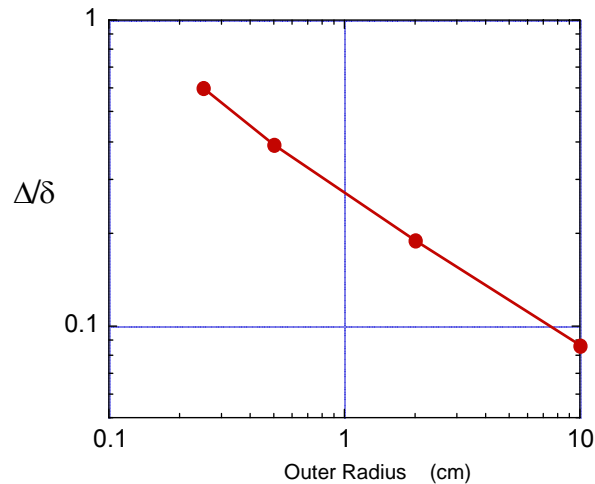
Figure 73. For larger spheres, resonance occurs when the shell thickness is a smaller fraction of the skin depth, other things being equal.
