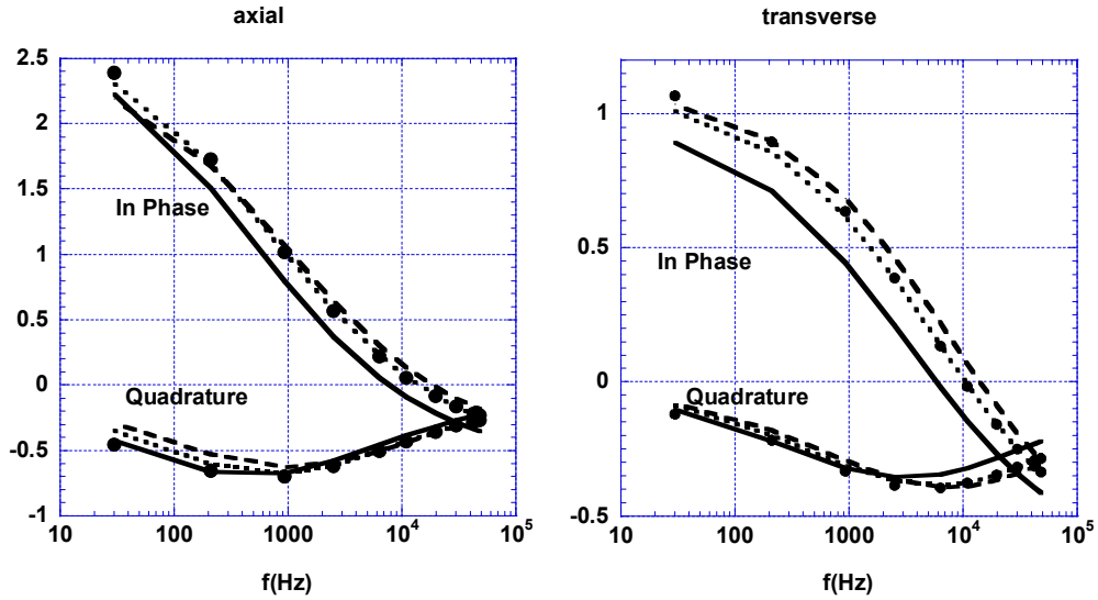
Figure 30. Measurements (solid markers) and responses obtained using the TSA algorithm, for a small steel cylinder. Solid lines: \mu_r = 55 , \sigma = 5.5 \times 10^6 S/m. Dotted lines: \mu_r = 95 , \sigma = 5.3 \times 10^6 S/m. Dashed lines: \mu_r = 95 , \sigma = 4.0 \times 10^6 S/m.
