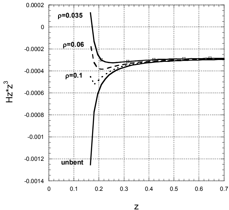
Figure 63. Axial scattered field from bent and unbent flattened ellipsoids, scaled by Z^3 , vs axial coordinate Z (m)
