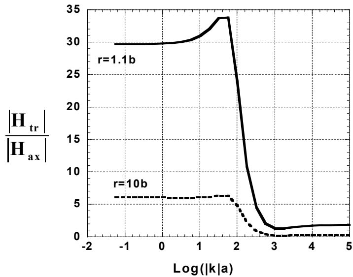
Figure 43. Magnitude of the ratio of transverse to axial response for 1x5 oblate spheroid at near and far field. \mu_r = 100
