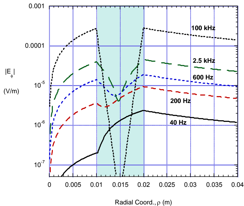
Figure 64. |E_\phi| , proportional to electric current, with an annulus interior (left area), the annulus wall itself (shaded region), and the exterior region (right area), for axial excitation at different frequencies. Non-magnetic, \sigma = 10^7 S/m.
