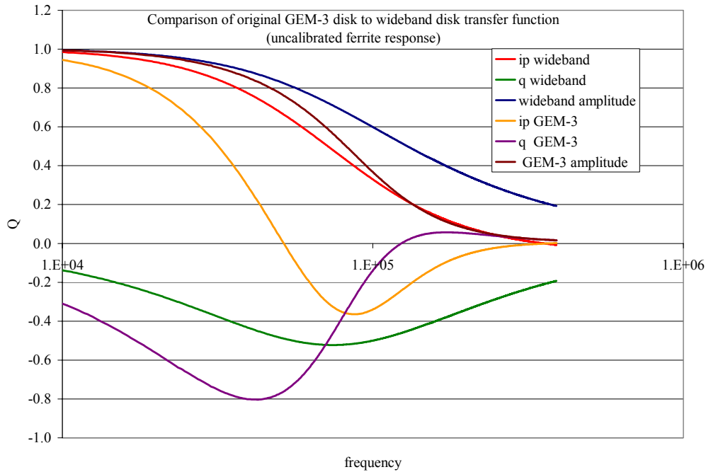
Figure 85. Theoretical coil frequency responses for the standard GEM-3 and the wideband GEM-3 coils, showing the greater attenuation above 100 kHz for the standard coils.
