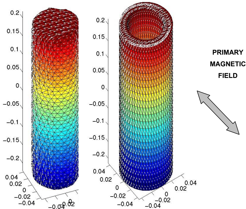
Figure 58. Solid cylinder and comparably sized cylindrical shell, with primary field impinging from the side, showing surface current currents (white arrows) at the PEC limit.
