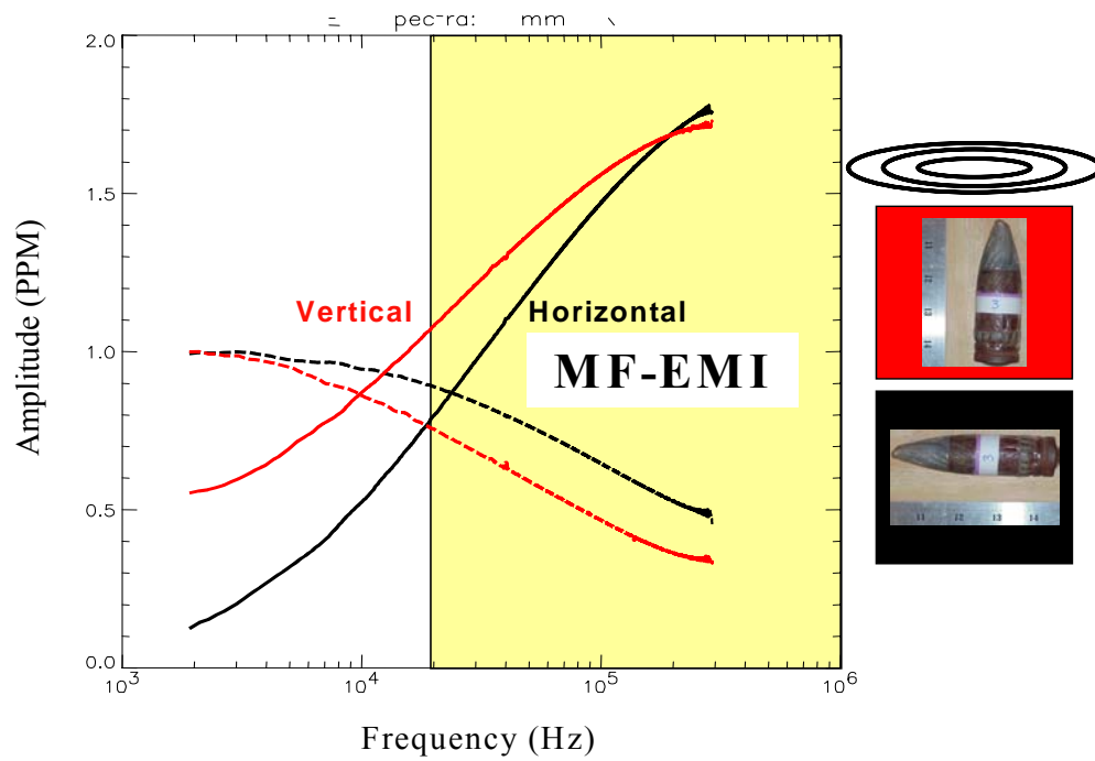
Figure 92. Measured response from 30 mm projectile, into MF-EMI range.
