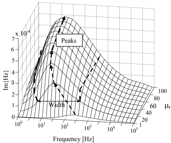
Figure 27. Quadrature component for spectral response of a long cylinder ( L/2a = 7 ), as a function of permeability. Axial excitation, \sigma = 5.5 \times 10^6 S/m
