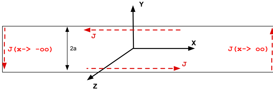
Figure 12. Schematic diagram of "parallel plate," infinite in the X and Z directions, with magnetic fields oriented only in the Z direction.
