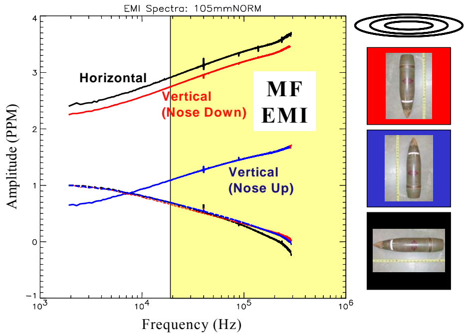
Figure 95. Measured response from 105 mm projectile, into MF-EMI range.
