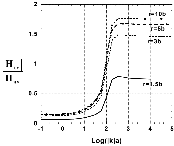
Figure 42. Magnitude of the ratio of transverse to axial response for 1x5 prolate spheroid, at different observation distances. \mu_r = 100
