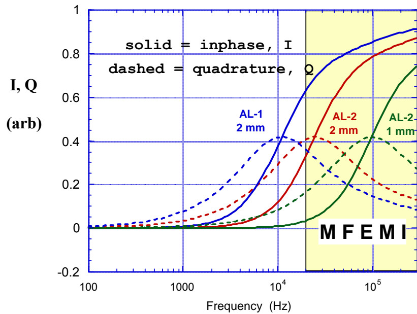
Figure 48. Normalized induced magnetic dipole moments for aluminum parallel plates of 1 mm and 2 mm thicknesses. Two different types of aluminum are considered: AL-1 ( \sigma = 2.9 \times 10^7 S/m) and AL-2 ( \sigma = 1.3 \times 10^7 S/m)
