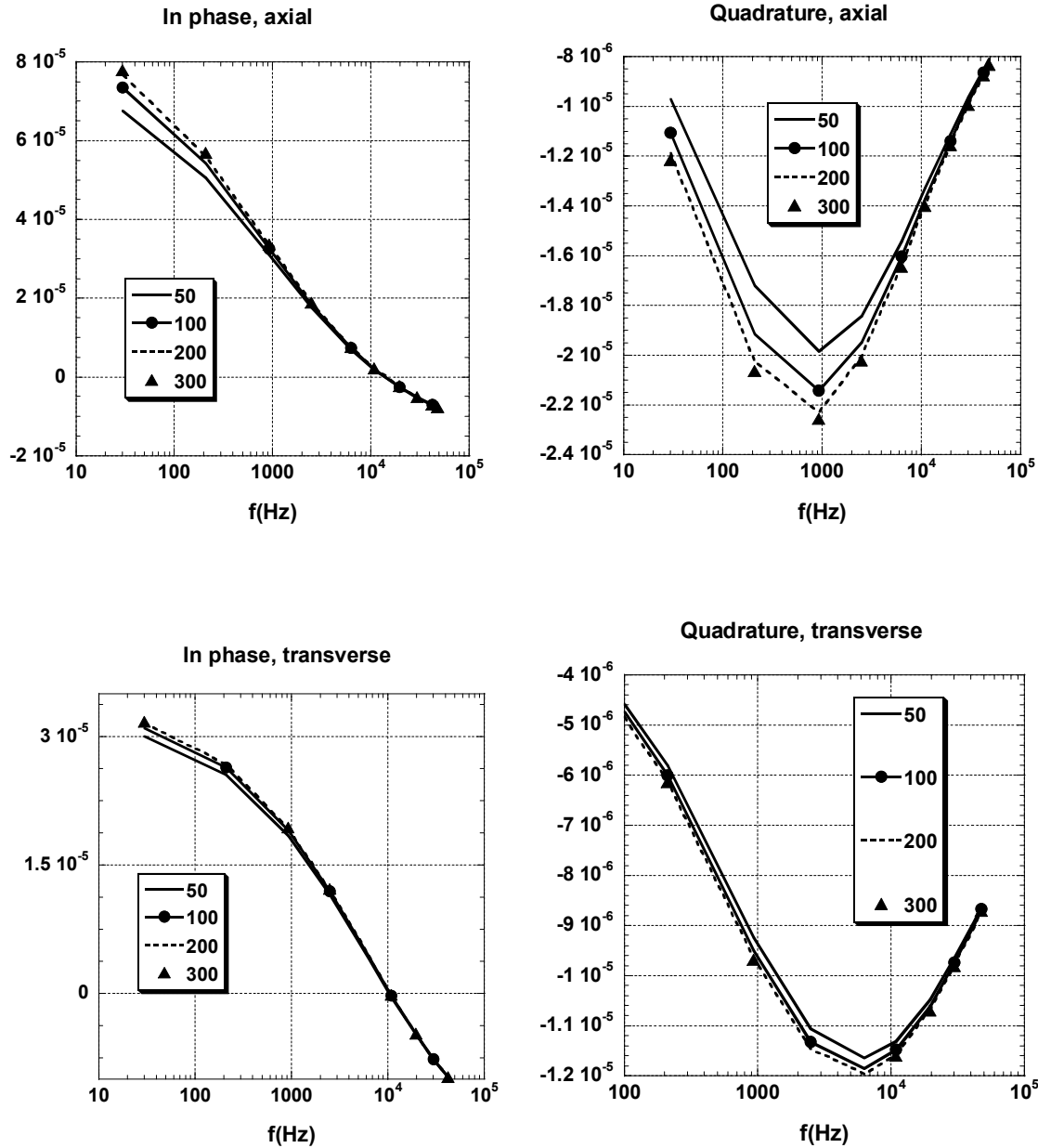
Figure 32. Scattered fields calculated for a 1x2 permeable cylinder, with \mu_r = 50, 100, 200, and 300, with \sigma adjusted in each case to maintain (\sigma/\mu_r) = (5/9) \times 10^5 S/m.
