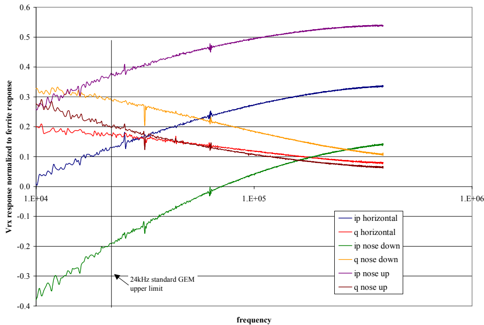
Figure 87. Extended frequency response of a 61mm mortar in three orientations, showing that the inductive limit (high-frequency inphase asymptote) is not reached until well beyond the GEM-3 bandwidth at the time of these experiments.
