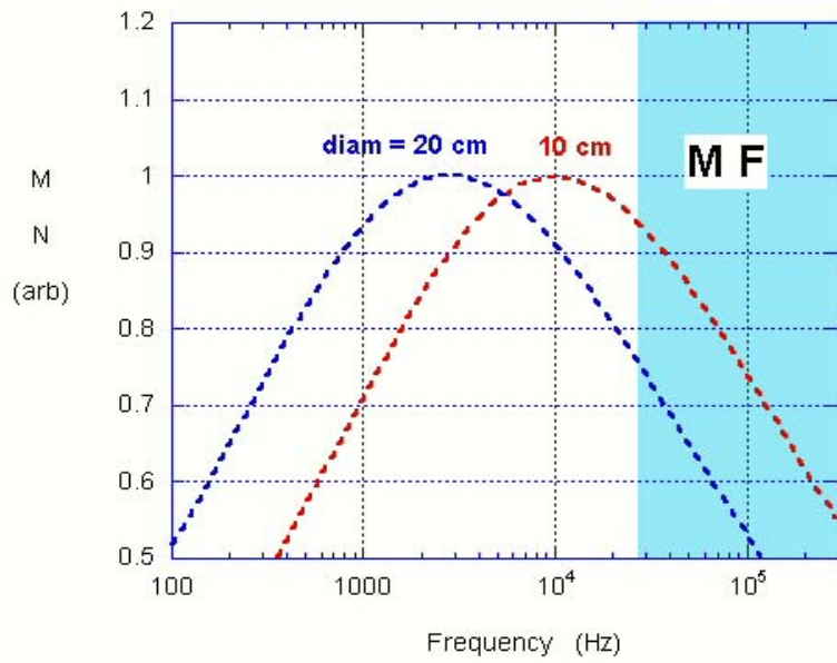
Figure 52. Comparison of Q components from 1 cm thick oblate spheroids, with AR = 10 and 20, for axial excitation, normalized by peak Q value.
