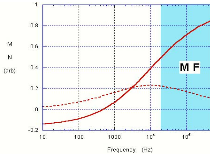
Figure 50. Normalized scattered field (dipole moment) for a magnetic oblate spheroid subject to axial excitation.
