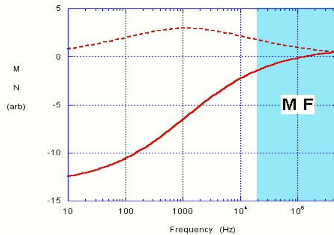
Figure 51. Same case as in Figure 50, but for transverse primary field.
