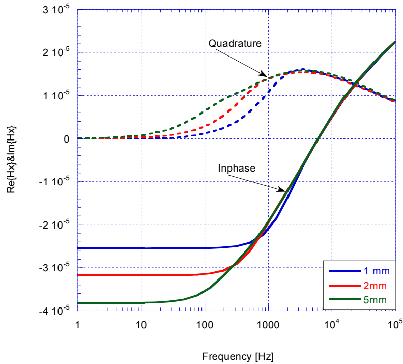
Figure 77. Secondary magnetic fields from the UXO shaped hollow shell, vs frequency, with \sigma = 4 \times 10^6 S/m, under transverse excitation, \mu_r = 50 . Different lines correspond to different shell thicknesses L_2 - L_1 = a_2 - a_1 .
