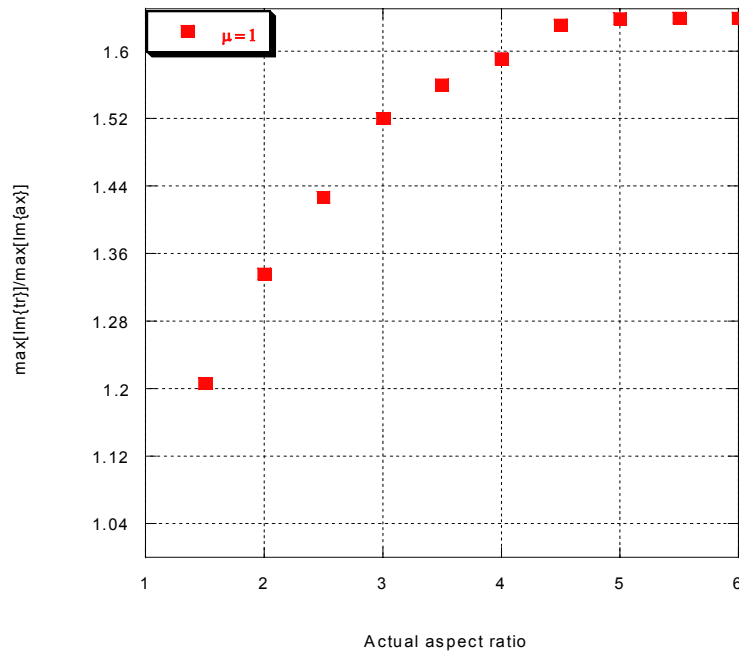
Figure 40. Ratio of magnitudes of the transverse to axial magnetic dipole moments vs actual aspect ratio, for cylinder with \mu_r = 1 .
