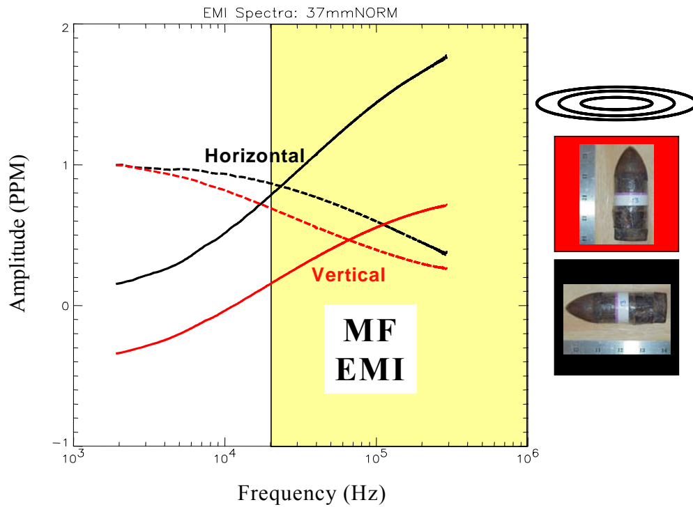
Figure 93. Measured response from 37 mm projectile, into MF-EMI range.
