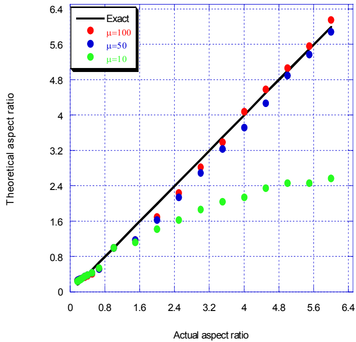
Figure 39. Theoretical aspect ratio from (69) vs actual aspect ratio, for different values of \mu_r . Top: cylinder, Bottom: spheroid.
