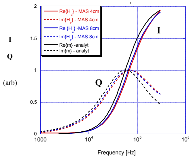
Figure 14. Normalized Inphase (I) and quadrature (Q) UWB EMI frequency responses from 4 mm thick stainless steel parallel plates ( \sigma = 1.4 \times 10^6 S/m, \mu_r = 1 ), showing approximate analytical result (analyt) and MAS results for circular disks with two different diameters.
