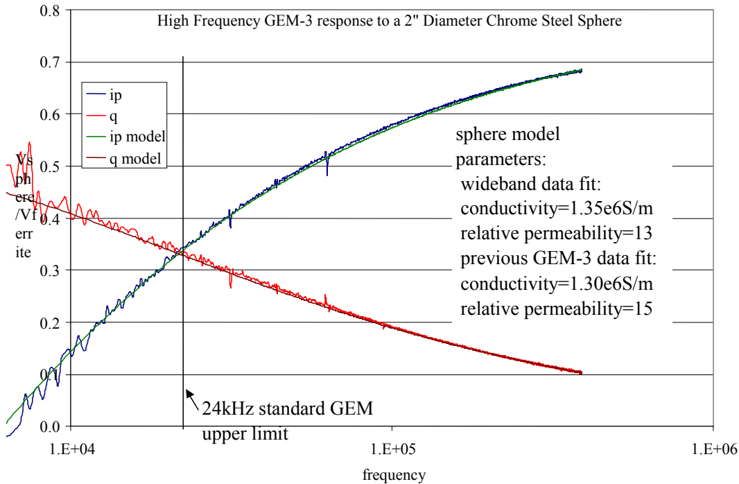
Figure 86. Measured spectrum of a chrome-steel sphere compared to a fit model.
