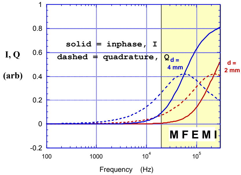
Figure 47. Normalized induced magnetic dipole moment for vertical plates of stainless steel ( \sigma = 1.4 \times 10^6 S/m) of thickness d .
