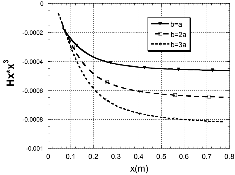
Figure 56. Broad side view of the three ellipsoids: Transverse case scattered fields, scaled by r^3 , for observation points and primary field orientation along the X axis.
