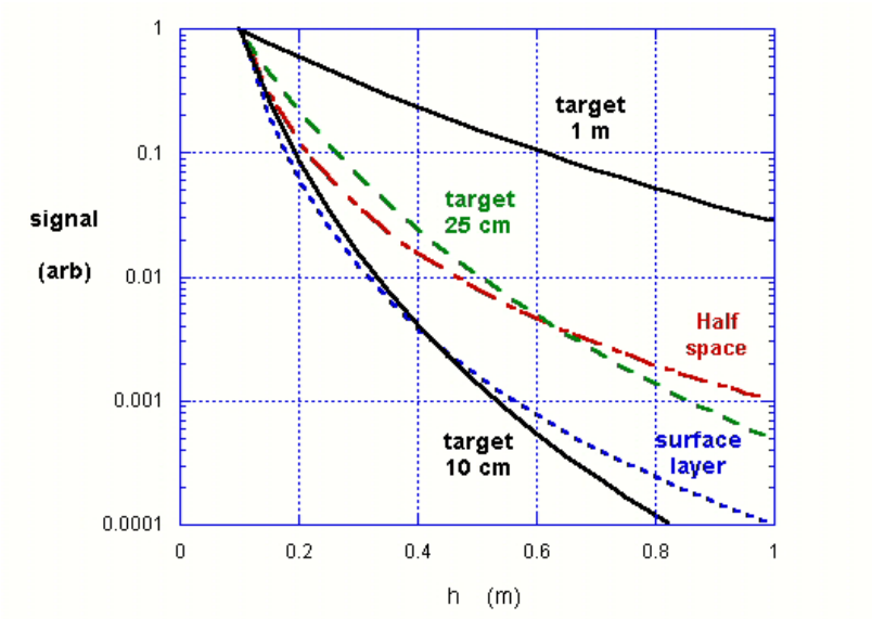
Figure 84. Received signals as a function of antenna height under dipole primary field, for surface and half space clutter layers, and from a target at indicated depths below ground surface.
