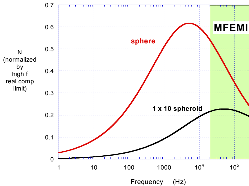
Figure 25. Analytically computed axial (broadside) responses of spheroids 5 cm in diameter, \mu_r = 100 , \sigma = 5 \times 10^6 S/m, for a perfectly spherical and a flattened (oblate) shape.
