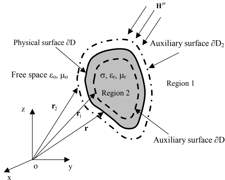
Figure 6. Geometry of scattering body, showing the relation of its physical and auxiliary surfaces
