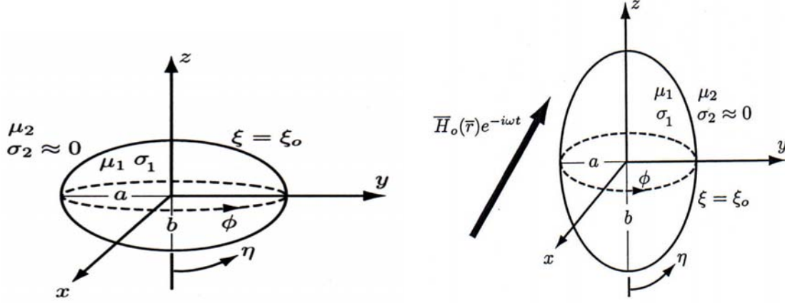
Figure 16. Geometry of an oblate spheroid (left) and prolate spheroid (right), with indication of the spheroidal coordinates (\xi, \eta, \phi) . We assume that \mu_2 in the soil is equal to \mu_0 .
