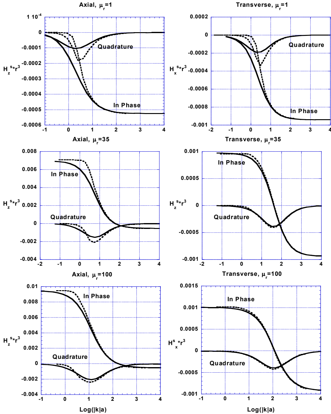
Figure 18. UWB frequency response for 1 x 6 prolate spheroid, with solid lines for TSA results and dashed lines for MAS, units on vertical axis are (A \cdot m^2) .
