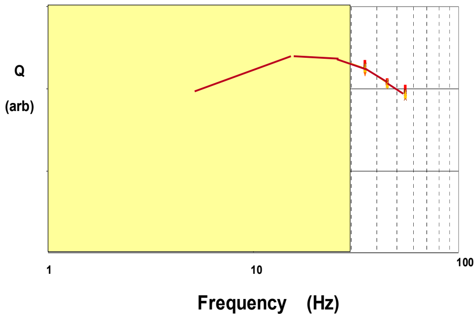
Figure 41. Quadrature frequency response of 105 mm projectile, nose down, measured with the experimental setup constructed during this project. VLF area is shaded on the left.
