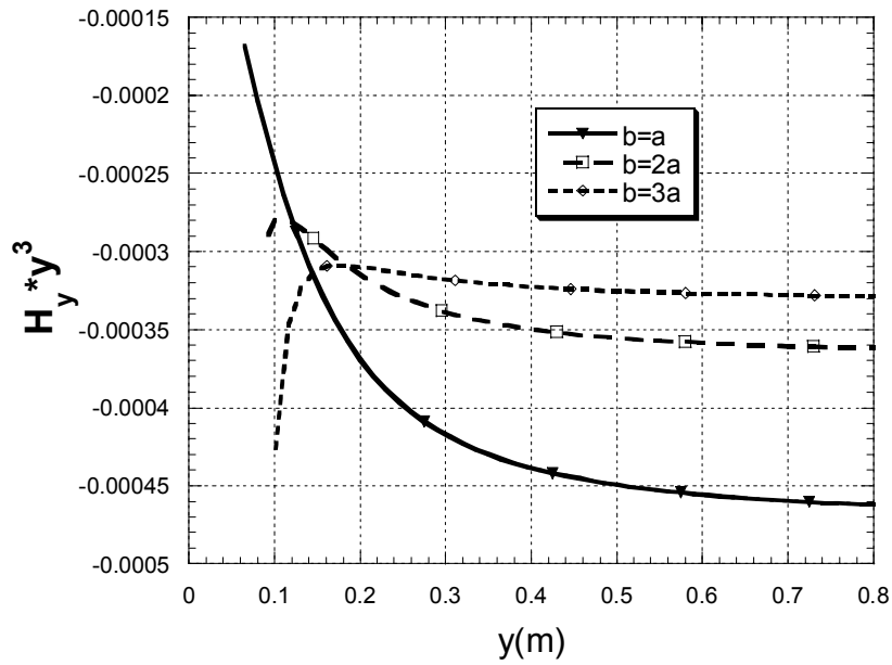
Figure 57. Narrow side view of the three ellipsoids: Transverse case scattered fields, scaled by r^3 , for observation points and primary field orientation along the Y axis.
