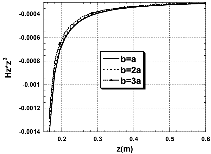
Figure 55. End view of ellipsoids: Scattered fields, scaled by r^3 , along Z axis, for the axial excitation case, for the set of three ellipsoids with different aspect ratios but same lengths and volumes.
