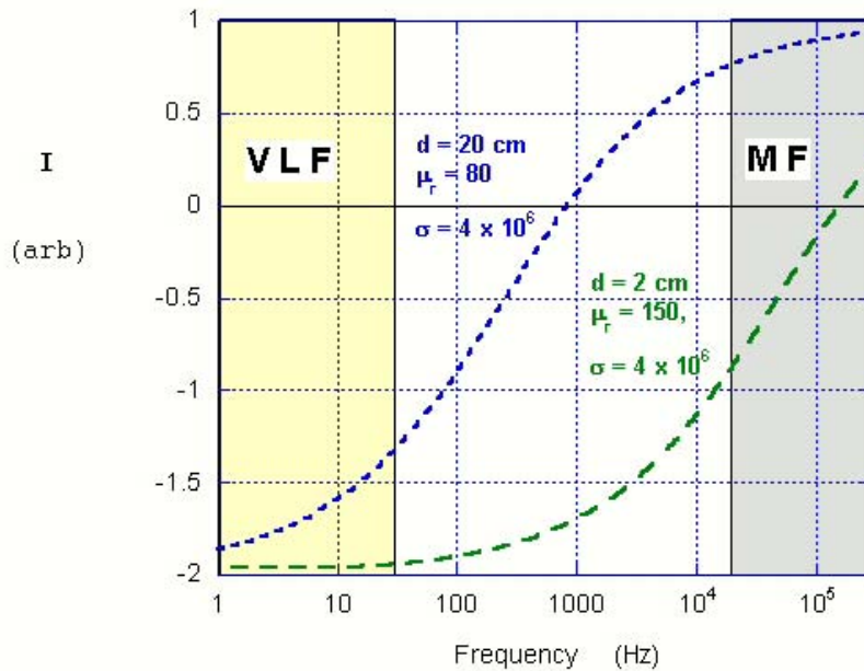
Figure 22. Inphase response patterns for the two magnetic cases in Figure 21.
