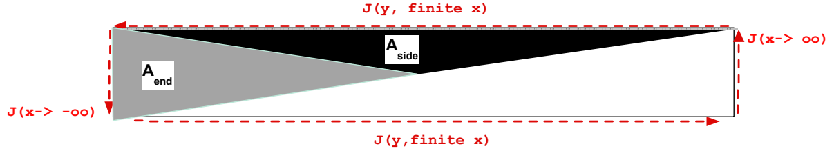
Figure 13. Cross section of a plate subjected to a primary magnetic field directed parallel to its sides, i.e. into the page, showing shaded areas that contribute equally to the induced dipole moment.
