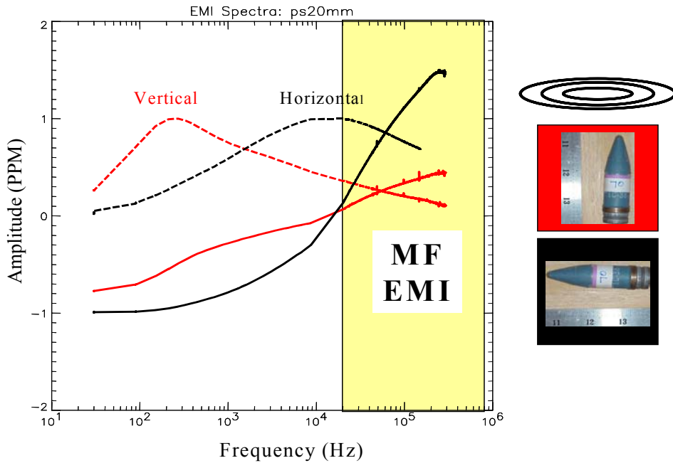
Figure 91. EMI data within five decades of frequency, including MF-EMI sub-band, for 20 mm shell.
