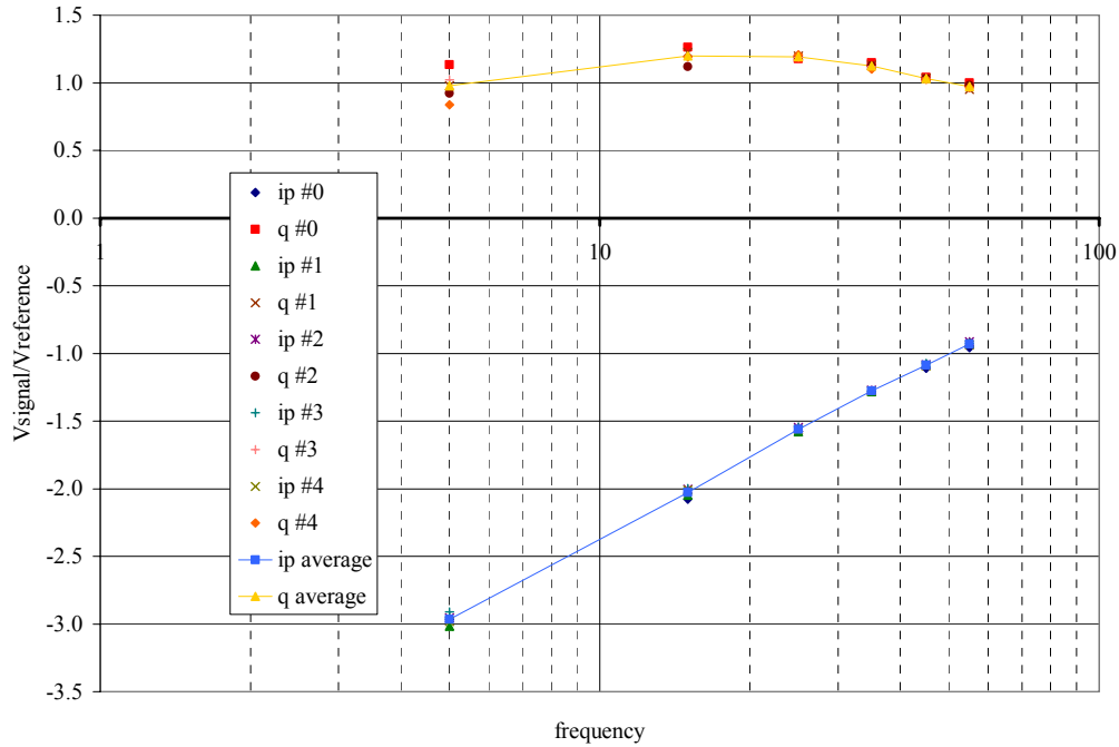
Figure 88. An example low-frequency measurement of the response of a 105 mm UXO, nose down, using the spectrum analyzer, with amplified drive current.
