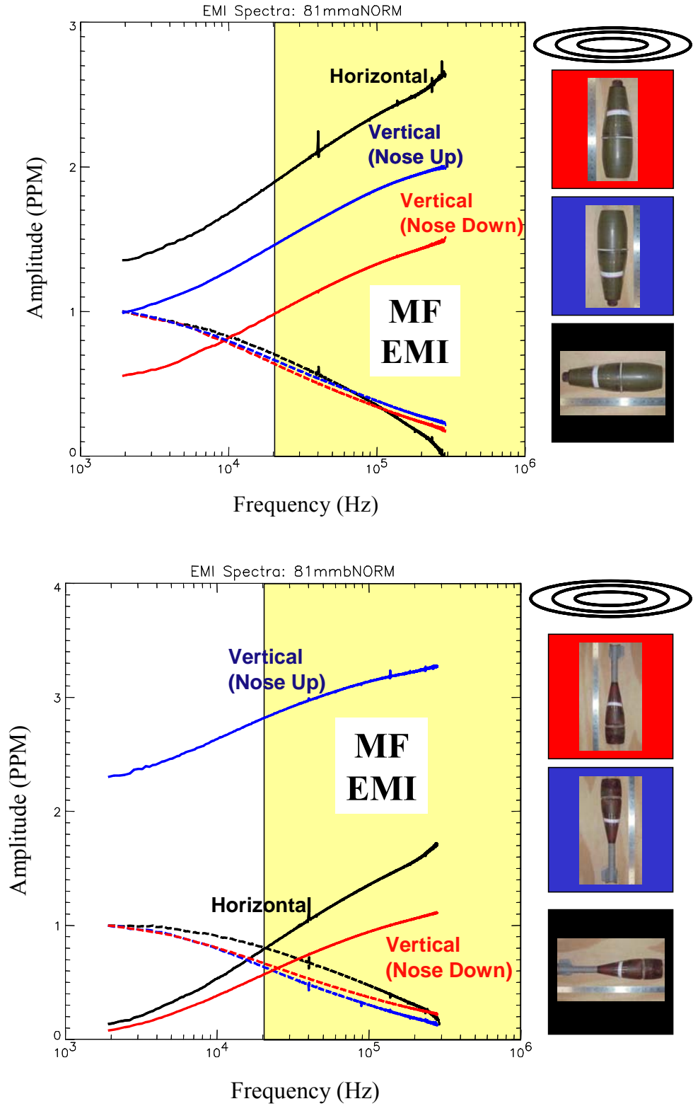
Figure 94. Measured response from 81 mm projectile, into MF-EMI range, with (bottom) and without tail (top).
