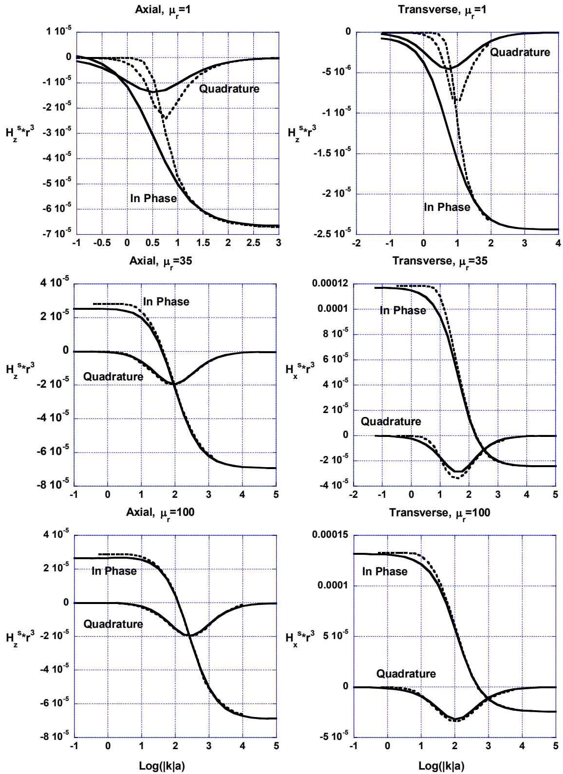
Figure 19. UWB frequency response for 4x1 oblate spheroid, with solid lines for TSA results and dashed lines for MAS. Units on vertical axis are (A m 2 ).
