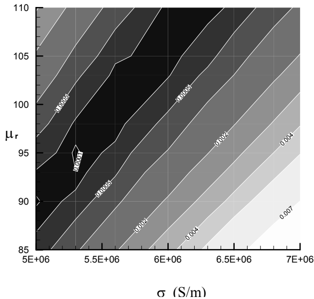
Figure 31. Error contours in (\sigma, \mu) space, for the small steel cylinder.
