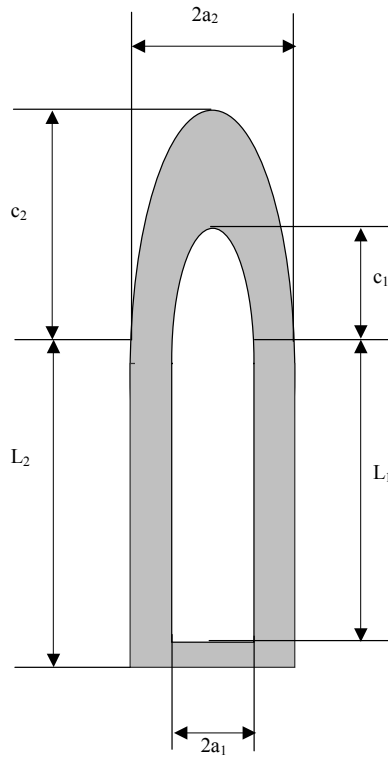
Figure 75. Hollow, UXO-like shape used in simulations
