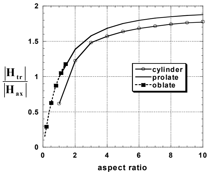
Figure 46. Ratio of computed transverse to axial response magnitude at the high frequency limit, for objects with different aspect ratios.
