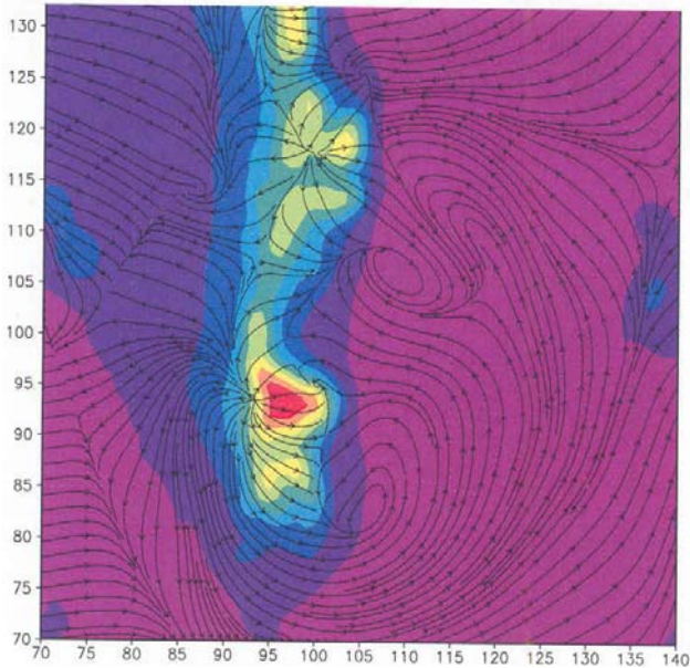
(b) streamlines
