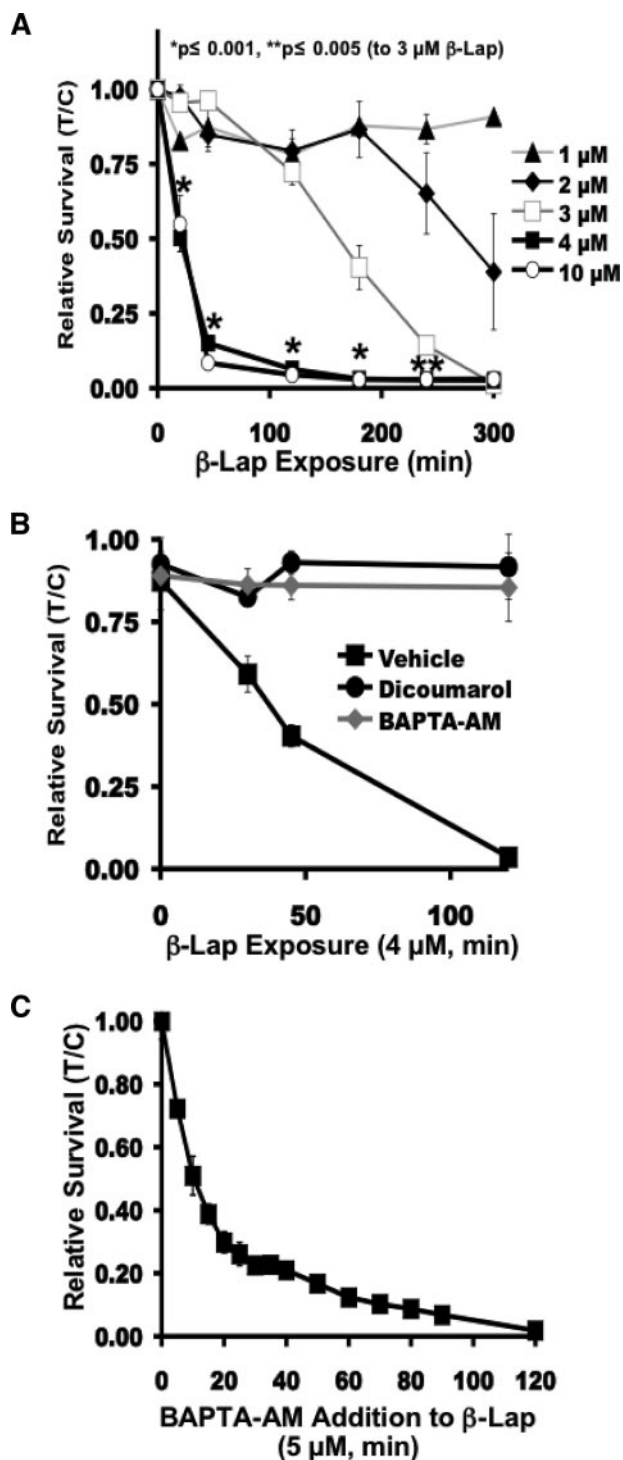
FIGURE 1. \beta -lap-induced cell death is time- and Ca 2+ -dependent. A–C, cell death was examined using relative survival assays in NQO1+ MCF-7 cells. A, cells were exposed to various doses of \beta -lap for different lengths of time to determine the minimal exposure time required for cell death. After drug exposure, media were removed and drug-free media added. Cells were then allowed to grow for an additional 6 days and relative survival, based on DNA content was determined by Hoechst 33258 staining as described under “Experimental Procedures.” Student’s t test for paired samples, experimental group compared with 3 \mu M \beta -lap (*, p \leq 0.001; **, p \leq 0.005). Prior studies using \beta -lap showed that relative survival assays directly correlated with colony forming ability. B, relative survival assays using MCF-7 cells treated with 4 \mu M \beta -lap alone, or in combination with 40 \mu M dicoumarol or 5 \mu M BAPTA-AM. C, MCF-7 cells were treated with 5 \mu M \beta -lap at t = 0. BAPTA-AM (5 \mu M) was then added to \beta -lap-treated cells at various times afterwards as indicated.
