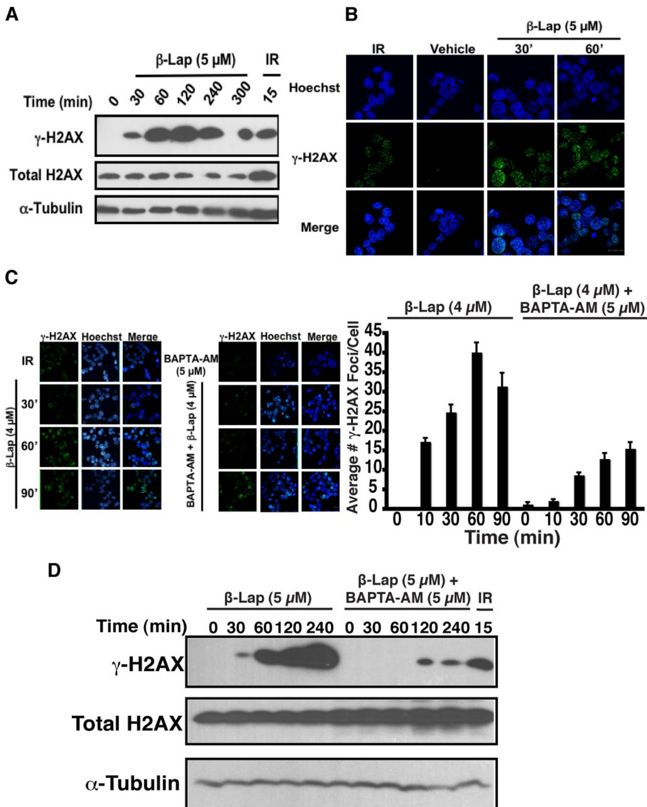
FIGURE 5. β-lap-induced γ-H2AX foci formation is abrogated by BAPTA-AM pretreatment. A, immunoblot analyses of γ-H2AX, total H2AX, and α-tubulin protein levels in whole cell extracts from MCF-7 cells exposed to β-lap for various times, or IR (5 Gy) harvested after 15 min. B, visualization of γ-H2AX foci in MCF-7 cells at various times after treatment with 5 μM β-lap or 15 min post-IR (5 Gy) by confocal microscopy. C, BAPTA-AM pretreatment followed by β-lap exposure abrogates γ-H2AX foci formation in MCF-7 cells as visualized by confocal microscopy. The number of γ-H2AX foci per cell was determined from at least 60 cells for each treatment group from four independent confocal experiments (means ± S.E.). D, immunoblot of γ-H2AX, total H2AX, and α-tubulin protein levels in whole cell extracts from MCF-7 cells exposed to β-lap for various times with or without BAPTA-AM (5 μM) pretreatment, or IR (5 Gy) harvested after 15 min.
