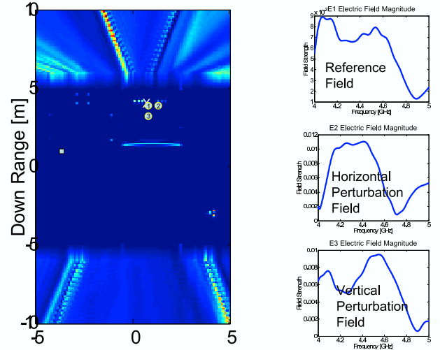
Fig. 8. The information gain field is computed by simulating the variability of the RF spectrum that a virtual transmitter in the vicinity of a pixel of interest (circle 1 in left panel) would generate at different locations at the exterior of the building. At right are the induced RF fields generated by a virtual transmitter at the reference position (circle 1), cross-range (circle 2), and range (circle 3) perturbations.
