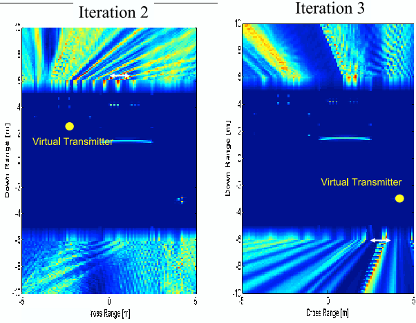
Fig. 9. Virtual transmitter locations and the induced information gain fields for iteration 2 and 3 of IRIS for the scenario illustrated in Fig. 5.
