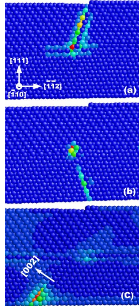
Fig. 3. An atomistic model containing a symmetric \Sigma 3 {111} twin, the interface of which is horizontal. Atoms are colored by their excess energy relative to perfect unstrained crystal with blue lowest and red, highest. (a). A perfect glide dislocation with b = 1/2 [101] is on the upper {111} plane in the model near the interface. (b) The model is subjected to pure shear stress such that the resolved shear stress on the dislocation is 1.77 GPa. The dislocation is moving across and then away from the twin interface onto the lower {111} planes. A Shockley partial with b = 1/6 [\bar{1}\bar{1}2] remains at the interface. (c) In response to a biaxial stress (tension or compression in a plane parallel to the interface) that exerts a resolved shear stress of 3 GPa, a dislocation moves away from the interface into the lower grain on a {200} plane, leaving a Shockley at the interface. Note that the Shockley has also moved slightly along the interface plane toward the right side of the model.
