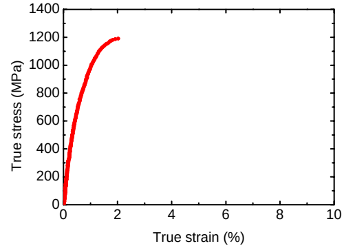
Fig. 6. True stress vs. true total strain curve for tensile tested Cu foils (20 \mu m) sputter-deposited at a deposition rate of 1.8 nm/s. The specimens have an average yield strength of 1.1 GPa and an elastic modulus of approximately 110 GPa.
