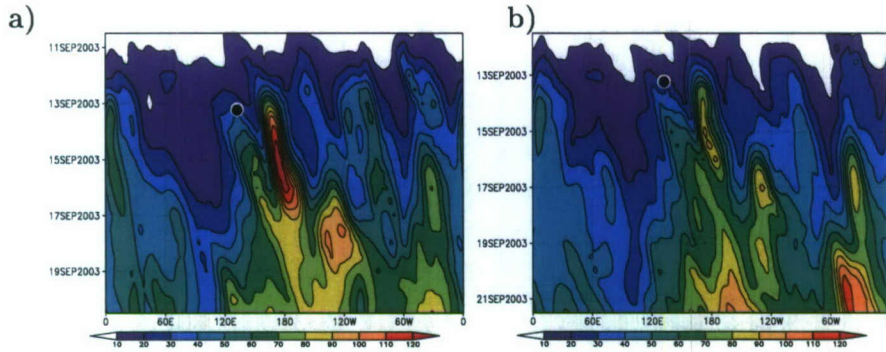
Figure 1: Standard deviation of 51 ECMWF ensemble members for 500hPa height during the ET of Typhoon Maemi (black dot). Forecast from a) 10 and b) 11 September 2003 1200 UTC.
