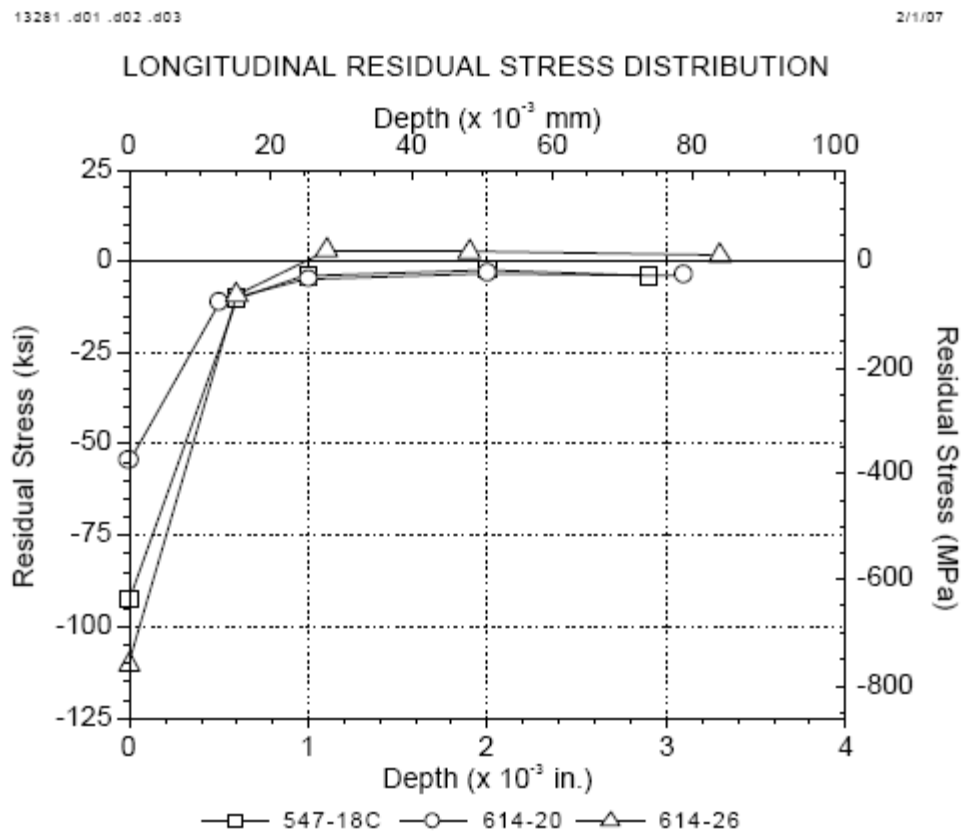
Figure 3: Longitudinal Residual Stress Depth Measurements, AF1410 Batch B Plates
