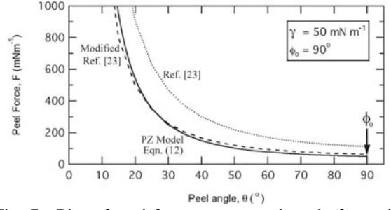
Fig. 7. Plot of peel force versus peel angle for a single spatula as given by Equation (12) using a crack energy of 50 mNm -1 as obtained by Huber et al. [Huber et al., 2005] and \phi_0=90^\circ . The dotted curve is the peel force of a single spatula as a function of peel angle obtained from reference [Tian et al, 2006]. The dashed curve is a fit of the peel force obtained from reference [Tian et al, 2006].
