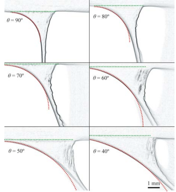
Fig. 4. Optical images of the peel zone region of the model tape peeling at a velocity of v \sim 0.03 \text{ mm/s} at peel angles of \theta = 90^\circ, 80^\circ, 70^\circ, 60^\circ, 50^\circ and 40^\circ . The corresponding model predictions for the curvature (dotted red curves) and the length of the peel zone (dotted green lines) are superimposed on the optical images.
