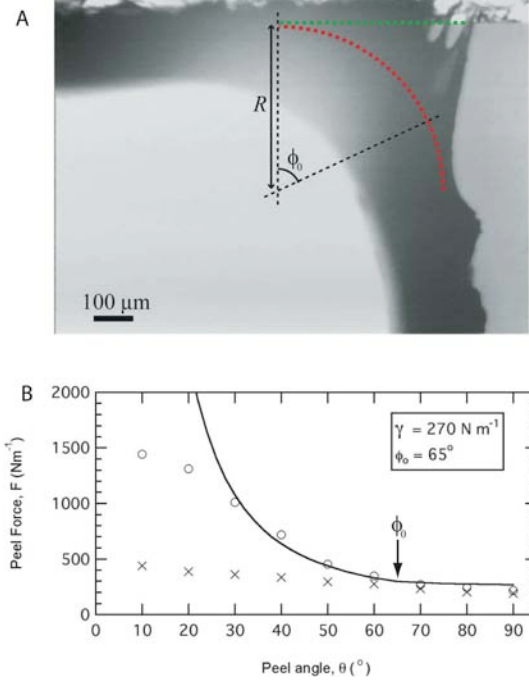
Fig. 5. (A) Optical image of a 90° peel of a composite tape composed of a layer of 3M Electrical tape with an additional later of 3M Scotch™ tape. (B) Plots of measured and theoretical peel forces versus peel angle for 3M electrical tape for a peel velocity of v \sim 0.5 mm/s. The solid line is the prediction of Equation (15). (X – data for a single layer of tape, O – data for the composite tape)
