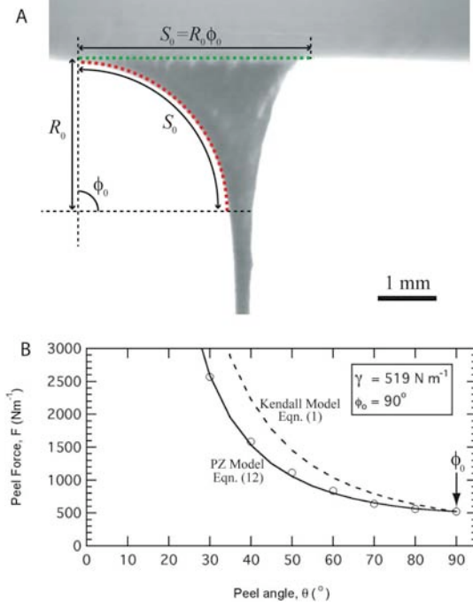
Fig. 3. (A) Optical image of a 90° peel of the model tape. The solid lines represent the predictions of the model for the curvature (dotted red curve) of the backing and the length of the peel zone (dotted green line). (B) Plots of measured and theoretical peel forces versus peel angle for a model tape consisting of a transfer tape adhesive on a transparency film backing at a peel velocity of v \sim 0.03 \text{ mm/s} . The solid line is the prediction of Equation (12). The dashed line is the prediction of Equation (1). In both cases, a crack energy of 519 \text{ Nm}^{-1} was used as defined at \phi_0 = 90^\circ .
