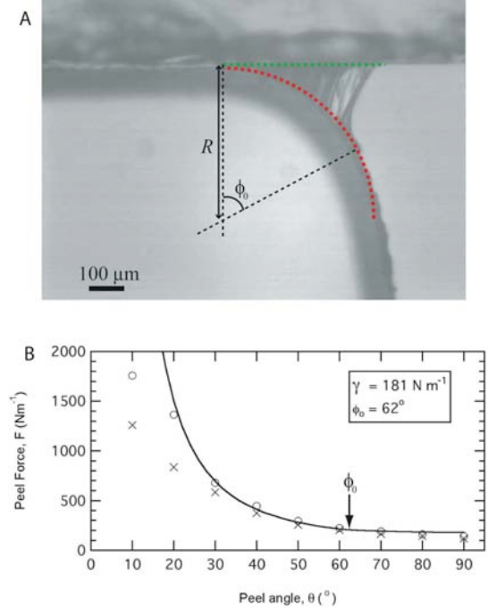
Fig. 6. (A) Optical image of a 90° peel of the composite tape composed of two layers of 3M Scotch™ tape. (B) Plots of measured and theoretical peel forces versus peel angle for 3M Scotch™ tape for a peel velocity of v \sim 0.5 mm/s. The solid line is the prediction of Equation [15]. (X – data for a single layer of 3M Scotch™ tape, O – data for the composite tape)
