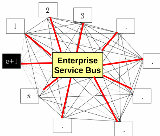
Figure 16. An n^2 Problem 11
