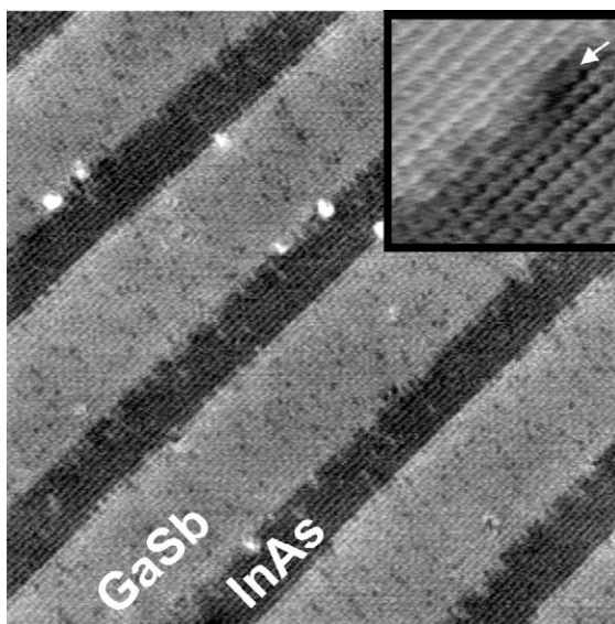
Fig. 5. XSTM image of a GaSb/InAs superlattice grown with P_b = 5.3 \times 10^{-6} Torr revealing the anion sublattice (60 nm × 60 nm). Dark (bright) atoms in GaSb (InAs) layer represent As cross-incorporation (Sb cross-incorporation). Inset: Close-up (7 nm × 7 nm) of an InAs/GaSb interface where a segment of GaAs interfacial bonds are observed (dark area indicated by the arrow).
