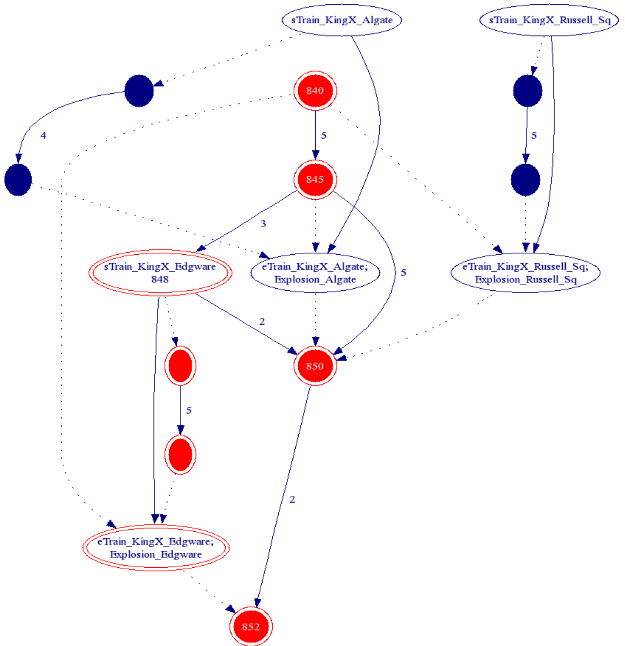
Figure 4.4: Inconsistency in the Point Graph
