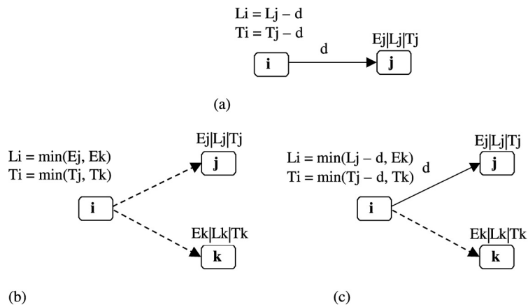
Fig. 7. Illustration of reverse pass.
