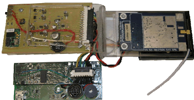
Figure 2: Open view of Ancile pager
