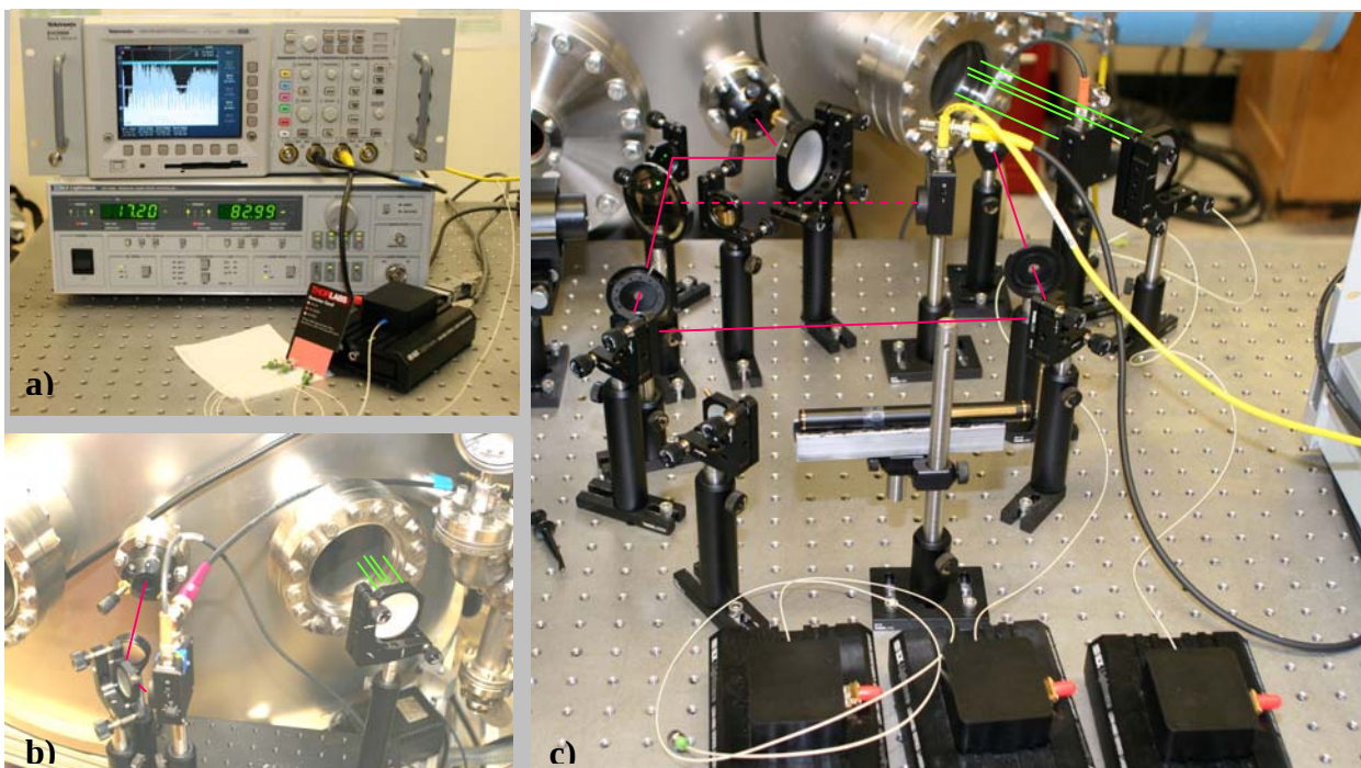
Figure 15. Laser absorption spectroscopy hardware. a) ILX system with sample spectra displayed on DSO. b) Detector mounted on across test cell in multipass configuration. c) Laser diodes, high finesse mirrors, and alignment optics.
