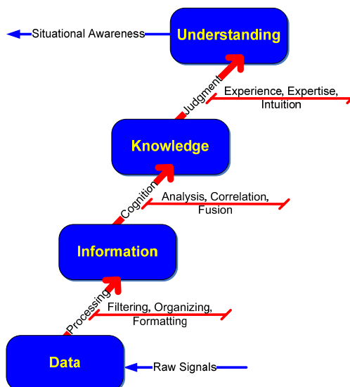
Figure 2: Cognitive Hierarchy
