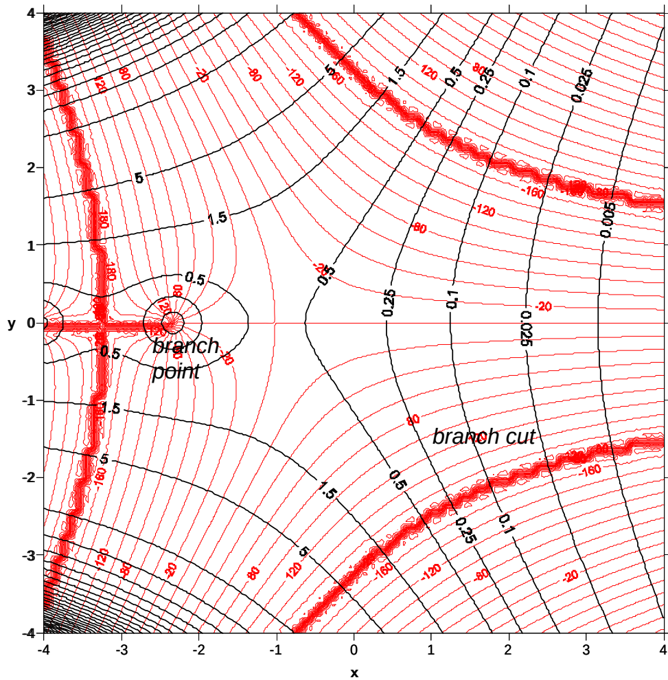
Figure B2. Ai(z) = |Ai|e^{i\phi} Airy function in the complex plane ( x, iy ) z = x + iy modulus black contour lines phase (°) red contour lines
