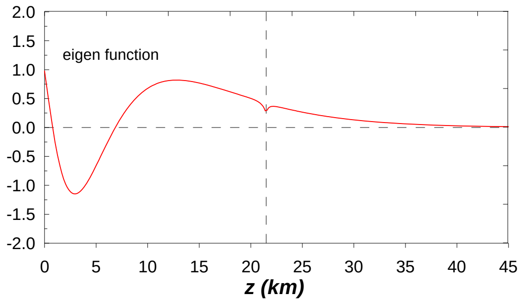
Figure 13c. As in figure 13a but for comparison of vertical eigenfunction \text{Re}(\tilde{\eta}_u/\tilde{h}) for \lambda = 40 \text{ km} . Vertical dashed line indicates turning point height z_t .
