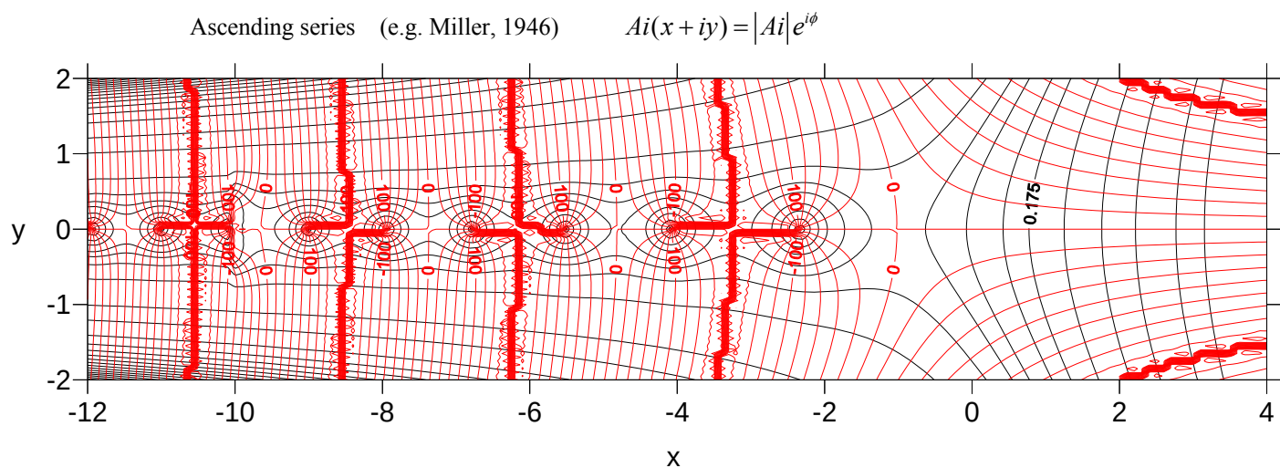
Figure B3. Comparison of machine and series solutions for the Airy function in the complex plane ( x , iy ). Contour analysis follows the same format as figure B2.
