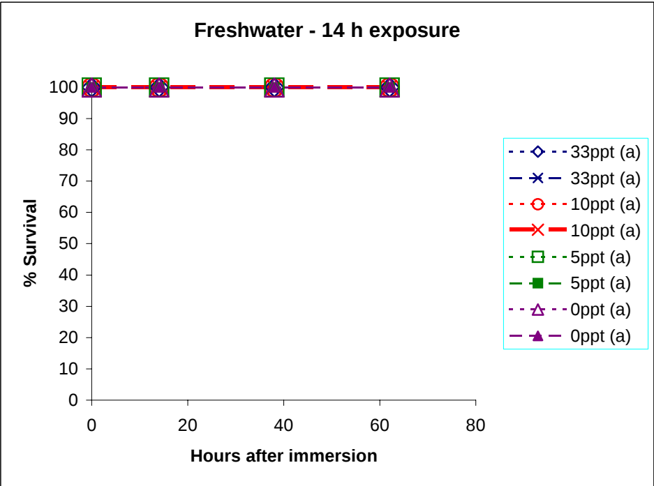
Figure 18. Test results for freshwater (14 h exposure)
