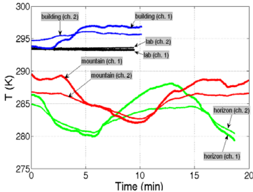
Fig. 1. Variation of the brightness temperature with time as measured in a clear day (afternoon) by detector 1 (thick lines) and detector 2 ( thin lines) for line of sight pointing toward (1) a building at 0.5 \text{ km} (blue), (2) a mountain at 6 \text{ km} (red), (3) the horizon (green), and (4) a blackbody at room temperature in the lab (black). Note: the two detectors measurements are simultaneous for each line of sight but the measurements for the three lines of sight are not simultaneous and were taken within \sim 1 hour.
