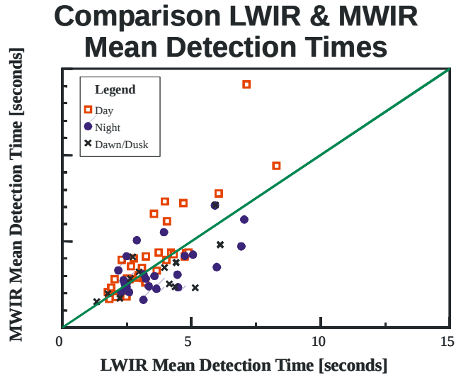
Figure 5. MWIR vs LWIR mean detection time for conventional targets in rural environment.
