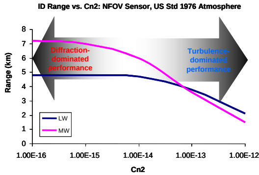
Figure 6. Example of modeled MWIR & LWIR range performance as a function of turbulence; and a characteristic day/night variation of C_n^2 in an arid/semi-arid climate 3
