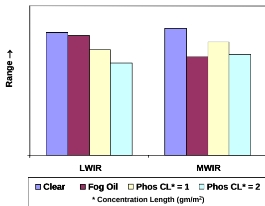
Figure 7. Modeled MWIR and LWIR range performance in smokes
