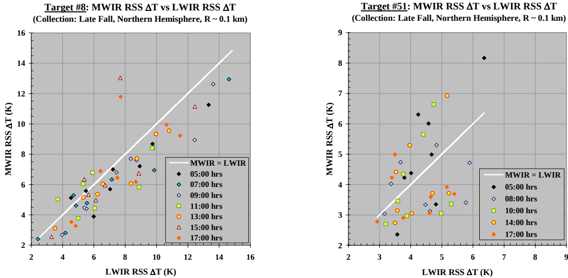
Figure 3. MWIR vs LWIR conventional target contrast
