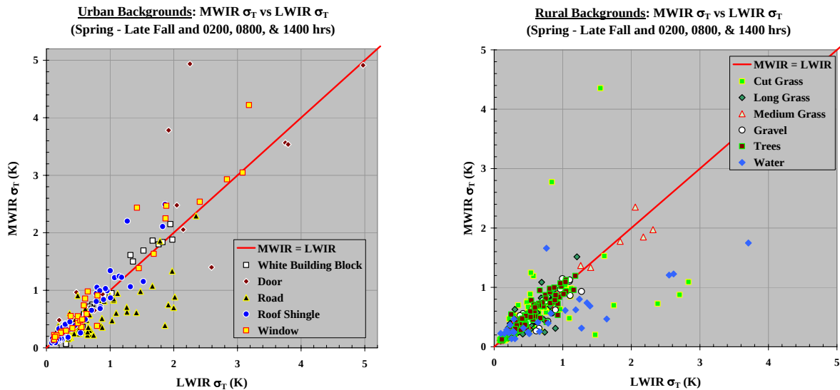
Figure 4. MWIR vs LWIR conventional and rural background contrast
