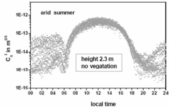
Figure 6. Example of modeled MWIR & LWIR range performance as a function of turbulence; and a characteristic day/night variation of C_n^2 in an arid/semi-arid climate 3
