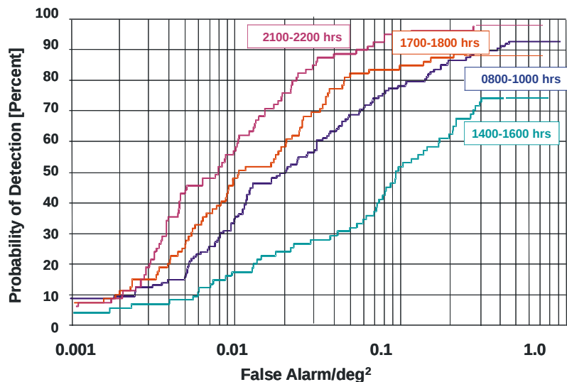
Figure 2. MWIR AiTR Performance as a Function of Time of Day
