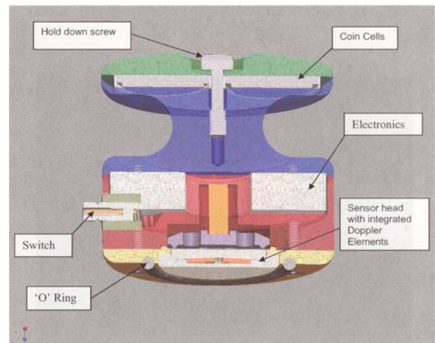
Figure 1. Dual-mode prototype stethoscope design.
