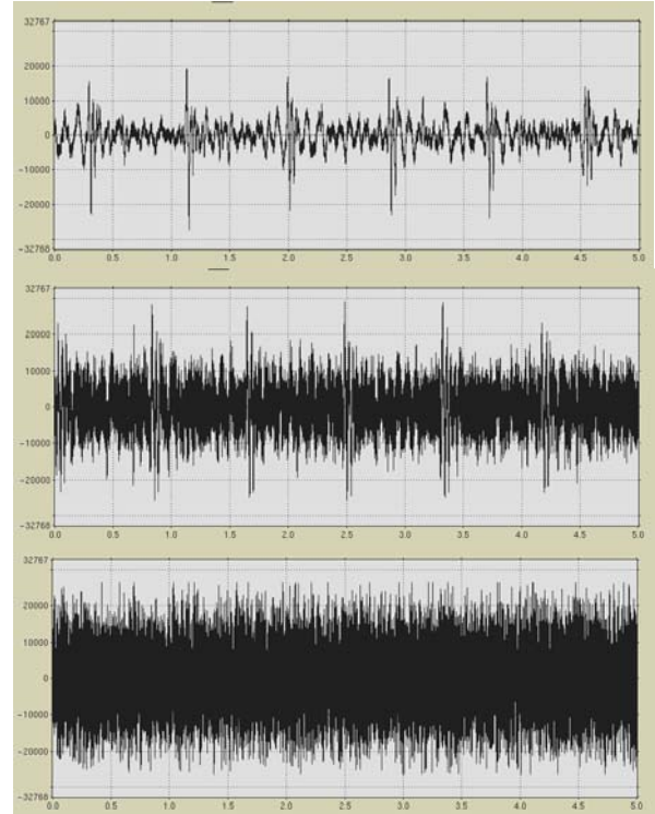
Figure 5. Same as Fig. 4, measured with the dual-mode prototype stethoscope in the passive electro-mechanical mode.
