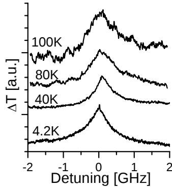
Fig. 1. Differential transmission at various temperatures (5 mW pump power). Scans were taken between 0.5 and 1 nm below LH line center
