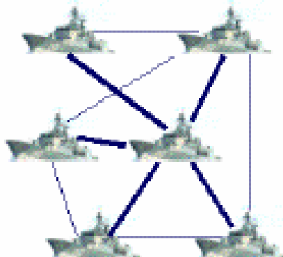
(a) Orchestrated
