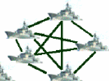
(c) Distributed
