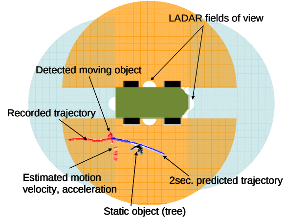
Fig. 2. Overview of the detection and tracking system . At the center of the figure is the vehicle (viewed from above), which carries four LADARs (one on each side).
