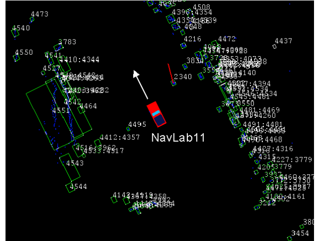
Fig. 4. A pedestrian, identified as Track 2340, moves at constant velocity. NavLab11 estimates the pedestrian's velocity while driving at 25 mph. The red line indicates the pedestrian's estimated velocity and direction. Other objects in the scene are identified by rectangular boxes. Raw scanner measurements appear as blue dots.
