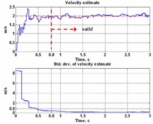
Fig. 3. Estimation of target velocity. A pedestrian walking at a constant speed of 2 m/s is tracked. The system reports a valid velocity estimate after 0.8 seconds, as shown in the top figure. The standard deviation of the velocity estimate, plotted in the bottom figure, is one of several criteria used to validate the track.
