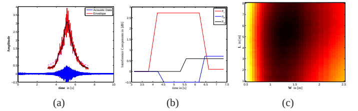
Fig. 5. Ford F150. (a) Estimated envelope by the interference components is shown with the solid line. The dashed line and the dotted line belong to the additive and multiplicative noise model results, respectively. (b) Estimated ES components are shown. According to the ES components, the vehicle is louder in the rear than front. (c) Estimated joint distribution of the vehicle dimensions around the solution.
