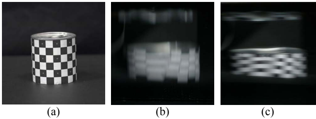
Figure 3: A cylindrical can with a checkerboard label (a) can appear both stretched and out of focus ((b) & (c)) when seen through our optical system. Photographing the scene with a wide lens aperture demonstrates the differing focal distances of vertical and horizontal image detail. With the lens focused at the distance of the spinning mirror, vertical image detail is in focus (b). With the lens focused an additional distance of 2r/\sin(2\alpha) beyond the mirror, horizontal detail comes into focus (c). This effect can be compensated for by using either a small aperture or corrective optics.
