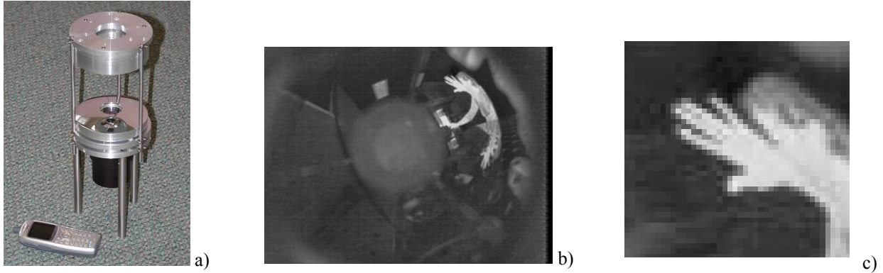
Figure 6. ViperView optics - experimental demonstration: a) experimental optical system; b) sample image produced by the camera; c) zoomed-in fragment of the same image showing pixel-limited resolution
