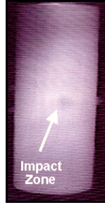
Fig. 7. Infrared imaging of the 3 ft-lb impact damaged tube specimen
