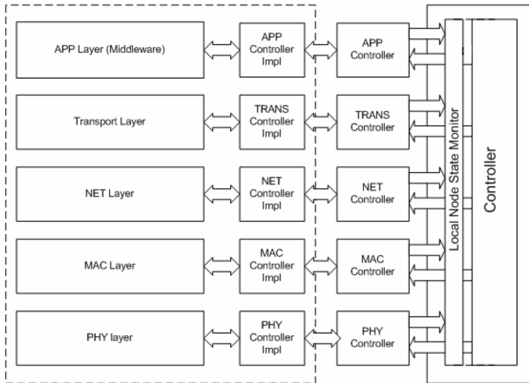
Figure 2. Cross-layer components with adaptable interfaces.
