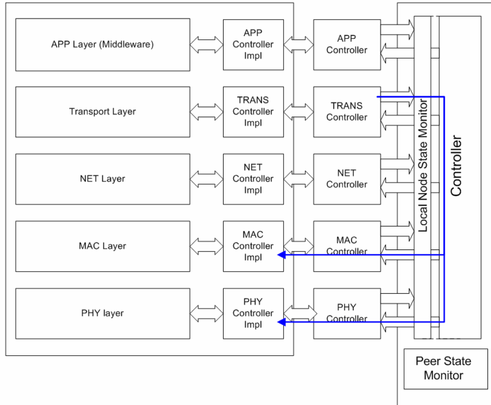
Figure 3. Routing layer or Middleware requirements coordinating wireless capacity (topology control and MAC scheduling)
