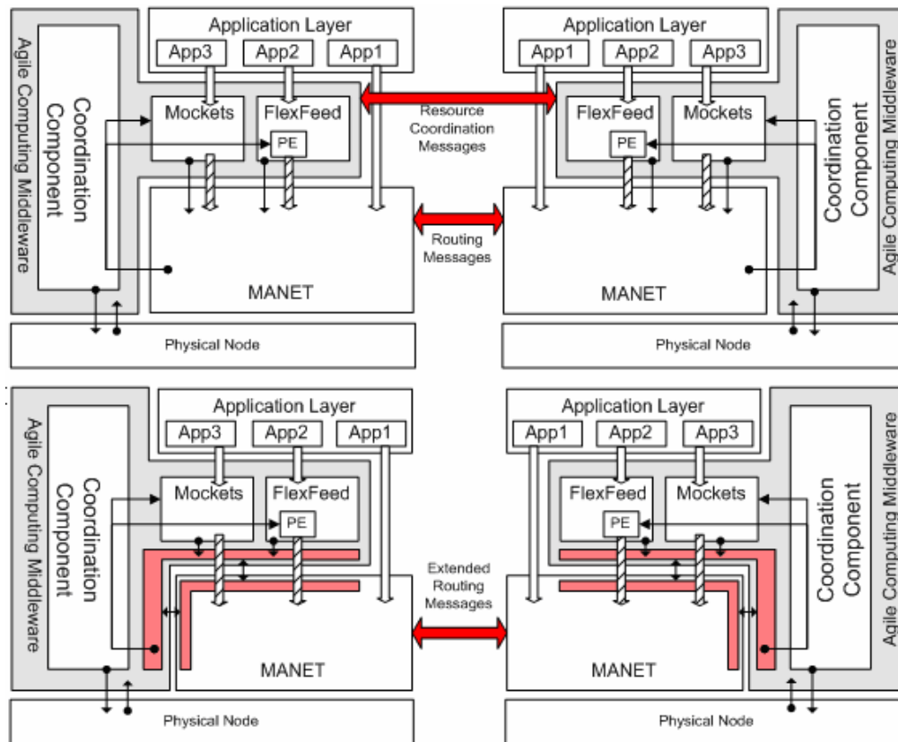
Figure 4. Integrating the current proof-of-concept implementation with the Agile Computing Framework
