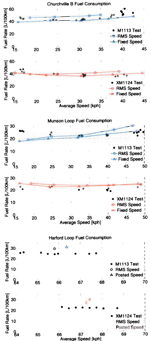
Figure 23. Fuel consumption plots from field tests at APG (stars) and improved GT-Drive bench runs (triangles and circles). 'RMS Speed' indicates speed command derived from the DCE-TOP experiment. 'Fixed/Posted Speed' indicates constant or piece-wise constant speed.
