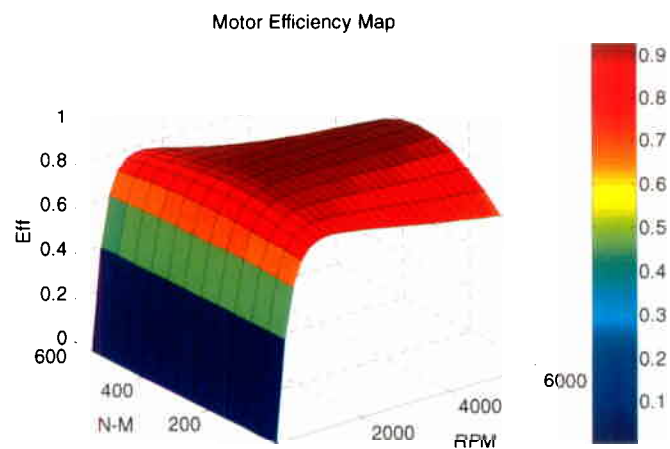
Figure 15. Efficiency map for the XM1124 electric motor.
