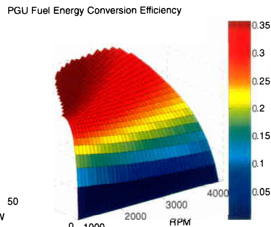
Figure 17. Efficiency map for the XM1124 PGU.
