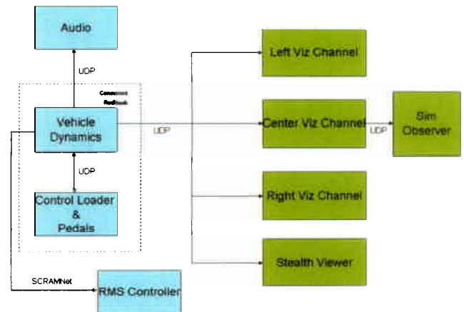
Figure 10. Top-level architecture.
