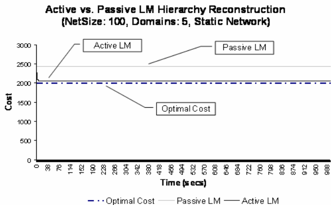
Figure 6. Ability of Active Maintenance to distributively reoptimize the quality of hierarchy as opposed to Passive Maintenance
