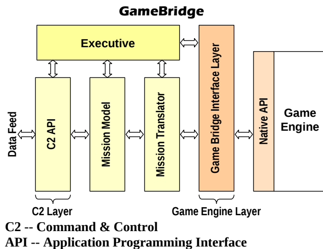
Figure 2 – GameBridge Architecture
